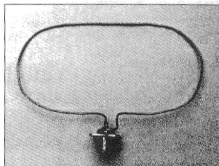
Photo C. Detail of a coupling loop.
