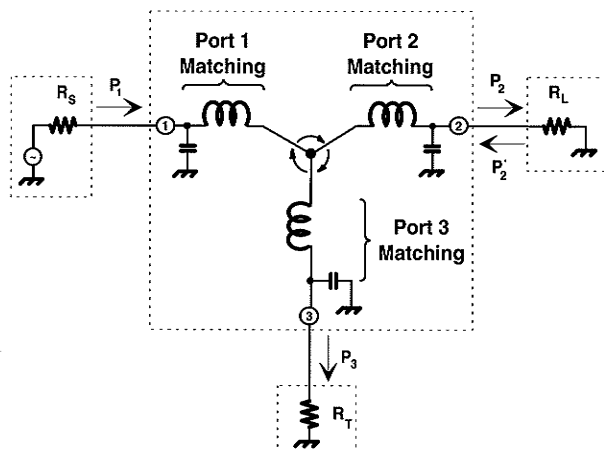
Figure 5 - Isolator = Circulator + Termination
