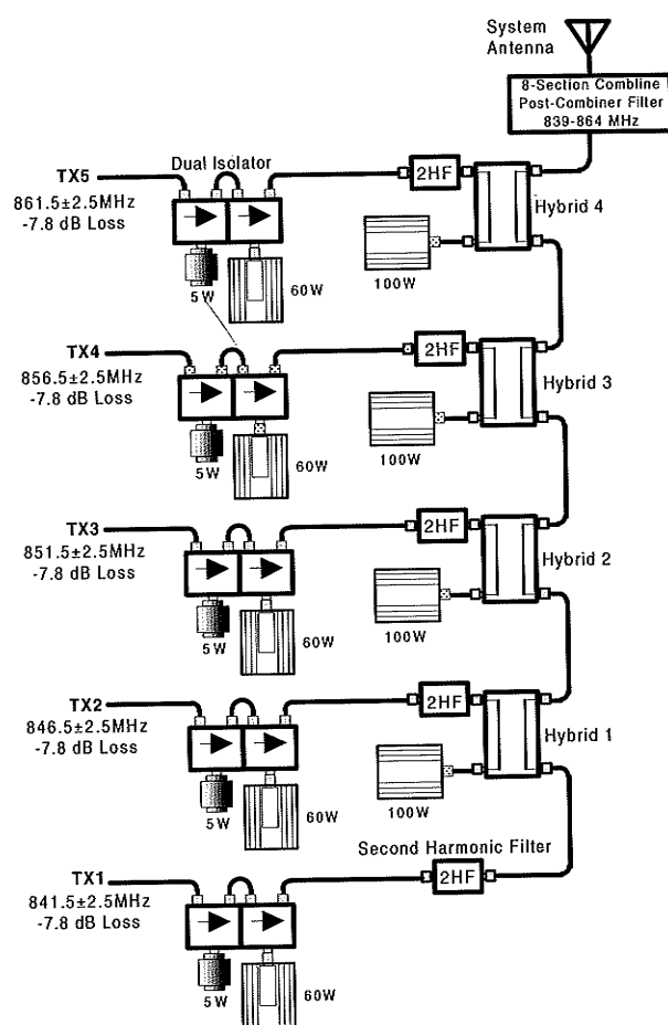
Figure 9 - 5-Channel Hybrid Combiner Model 431-90-92307
