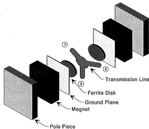
Figure 2 - Y-Junction, Distributed-Parameter Circulator Construction
