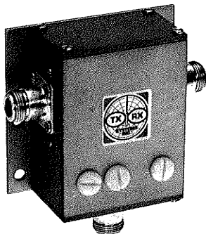
Figure 3 - 450-470 MHz Distributed-Parameter Circulator, Model 81-70-15-00
