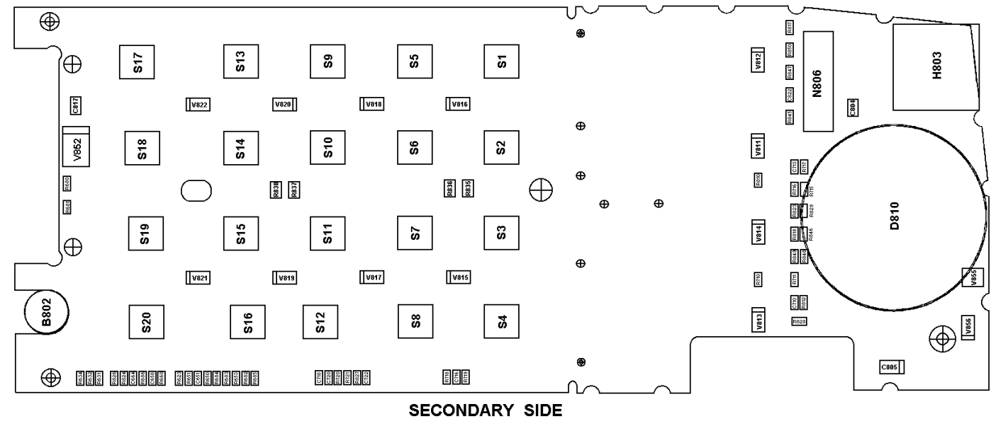
LOGIC BOARD ASSEMBLY 1078 ROA 117 2224
