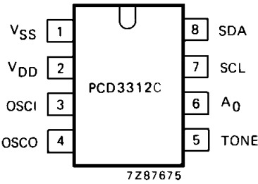
Lead Identification & Pin Out
