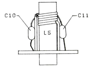
ASSY. FOR L5 C10 AND C11
