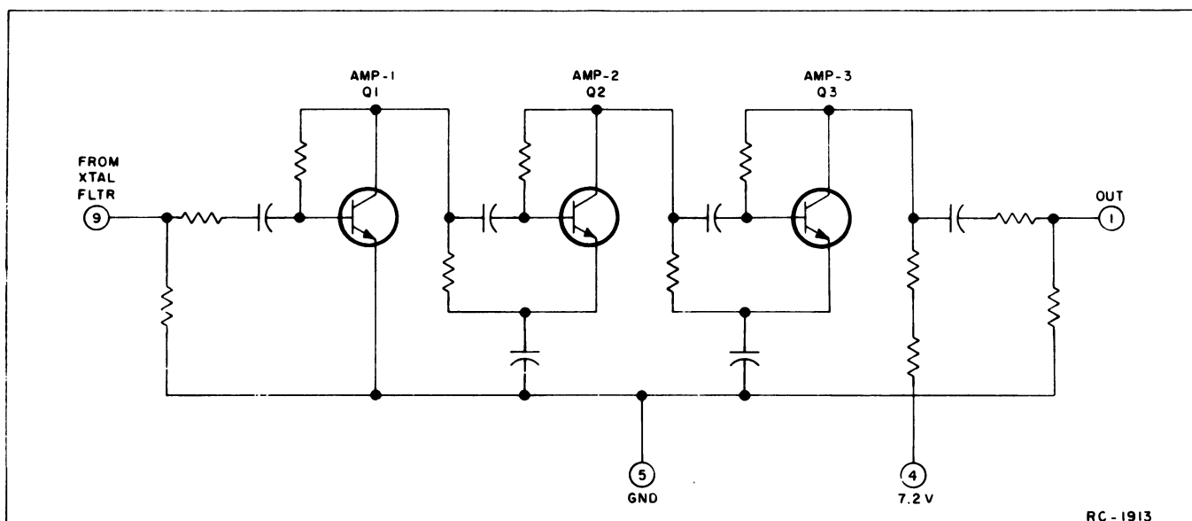
Figure 4 - Typical IF Amplifier Circuit
