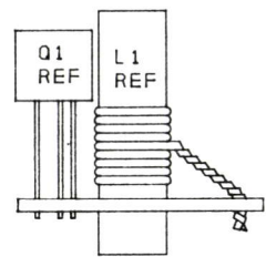
ASSY. FOR L1 AND Q1
