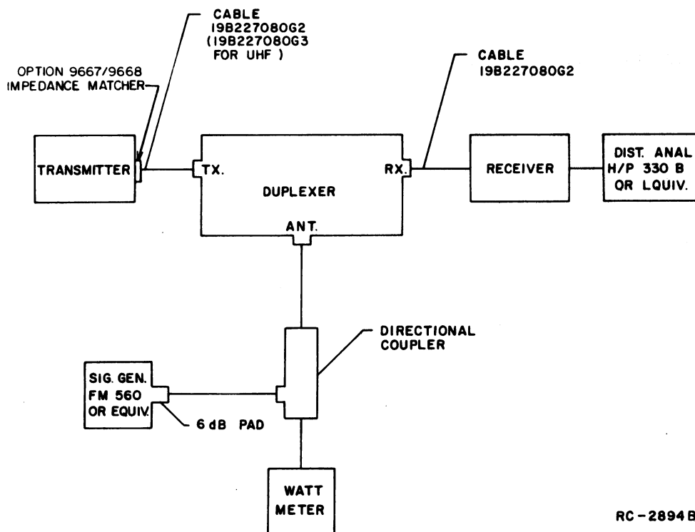
Figure 11 - Connections for Testing Duplexer
