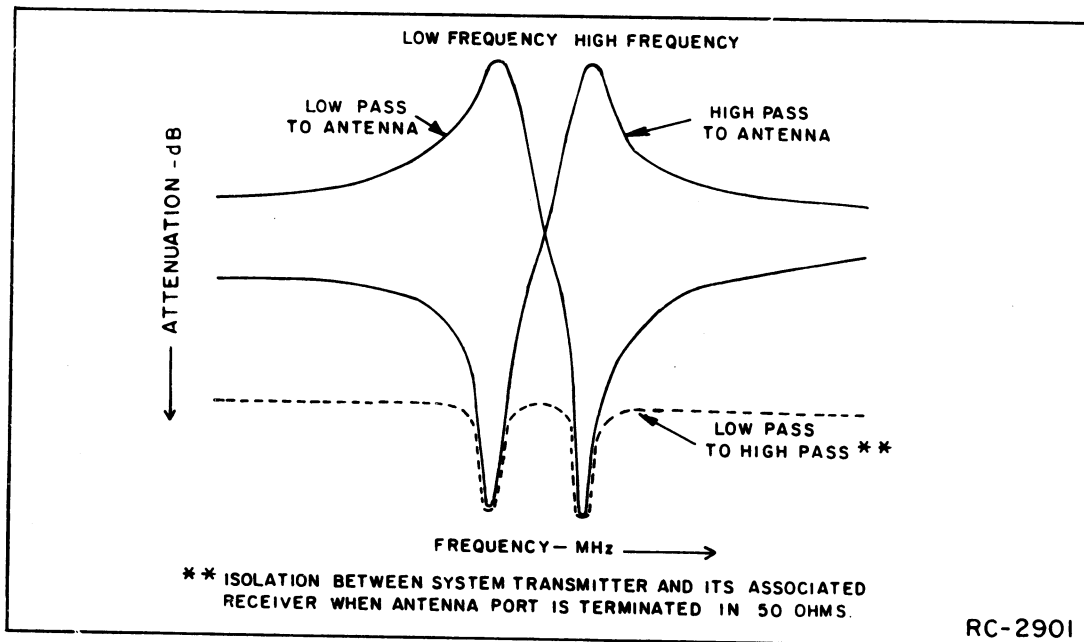
Figure 2 - Typical 19C307166 Duplexer Response
