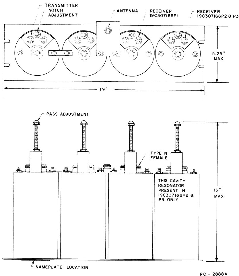
Figure 5 - Phelps Dodge Duplexer
