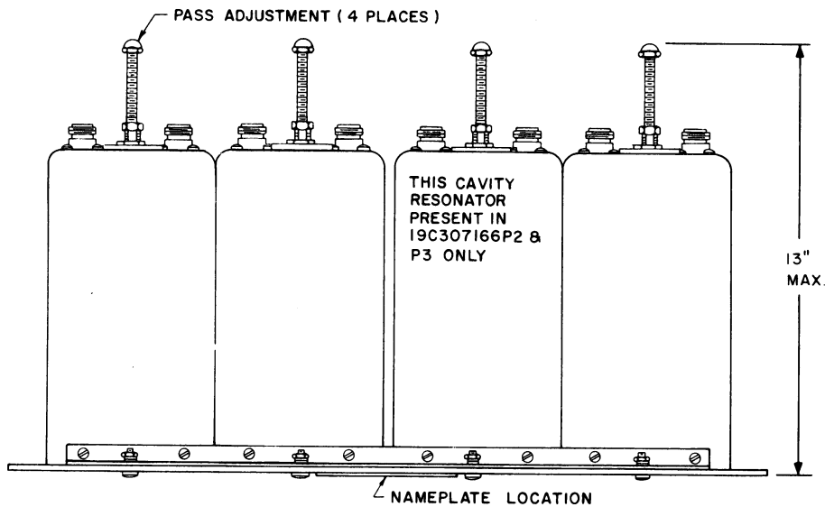
Figure 7 - DB Products Duplexer
