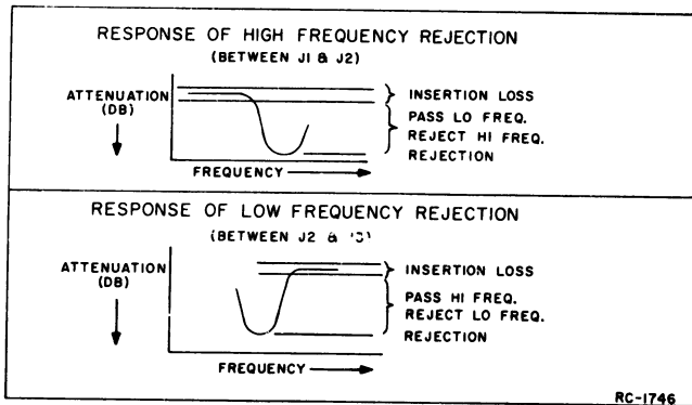
Figure 1 - Typical 19D402955 Duplexer Notch Response
