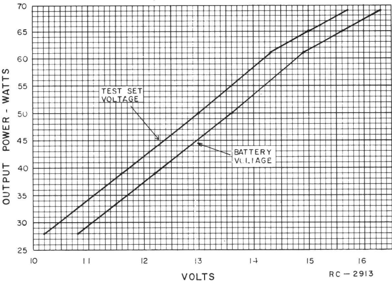
Figure 5 - Power Output Setting Chart
