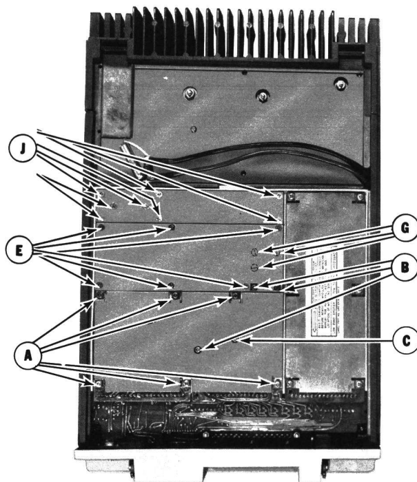
Figure 3 - Disassembly Procedure (Bottom View)
