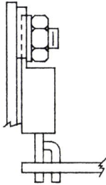
TYPICAL MOUNTING FOR Q901, Q916 AND Q917
