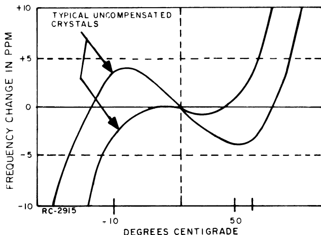
Figure 5 - Crystal Characteristics
