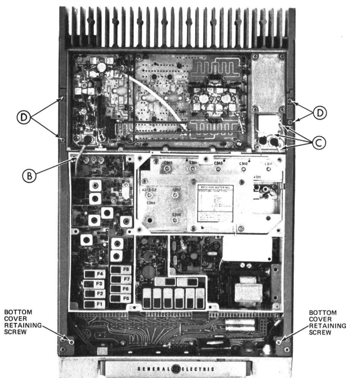
Figure 4 - Disassembly Procedure
