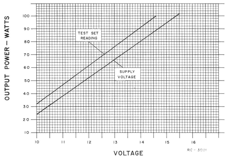
Figure 8 - Power Output Setting Chart
