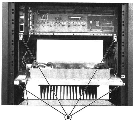
Figure 3 - Access to Power Amplifier Rear View
