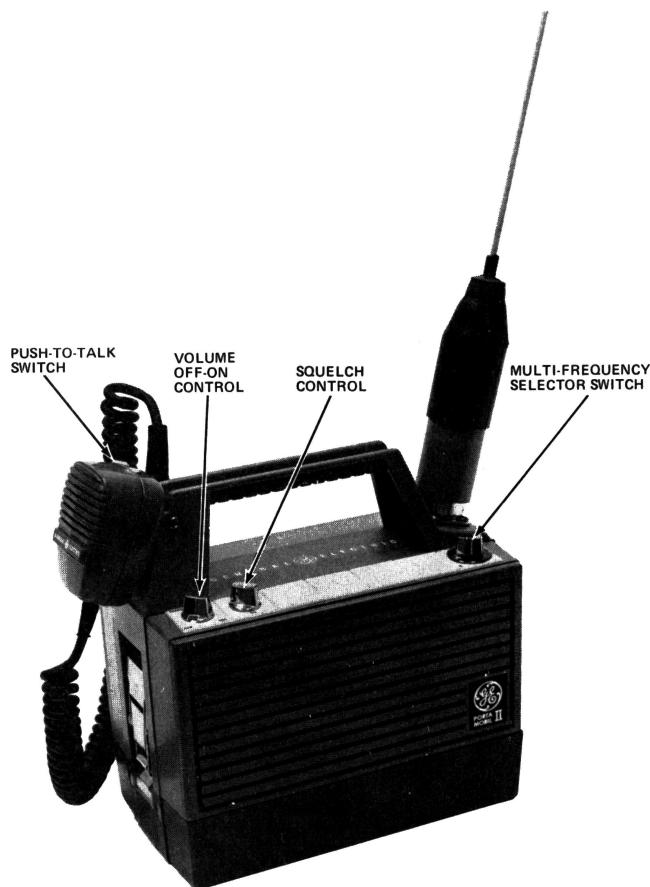
Figure 3 - Operating Controls
