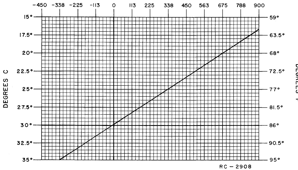
Figure 4 - Frequency Offset Chart
