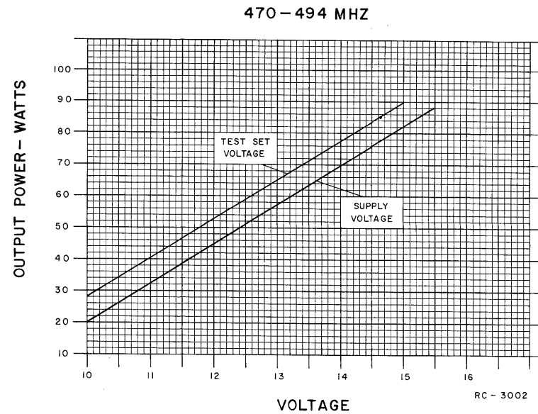
Figure 6 - Power Output Setting Chart
