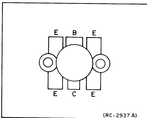
Figure 3 - Q203, Q4205 and Q4206 LEAD IDENTIFICATION
