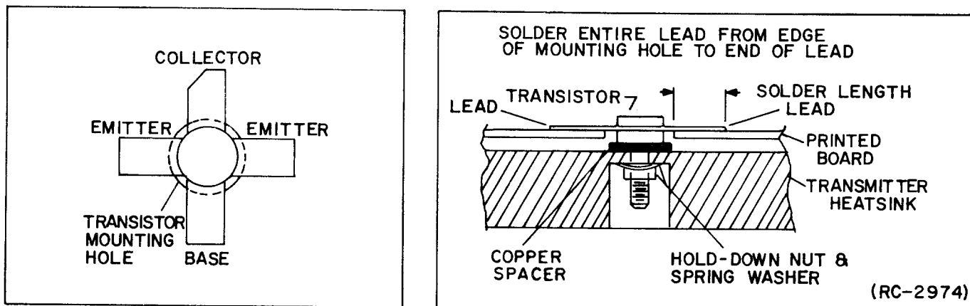
Figure 2 - Q202 Lead Identification and Mounting
