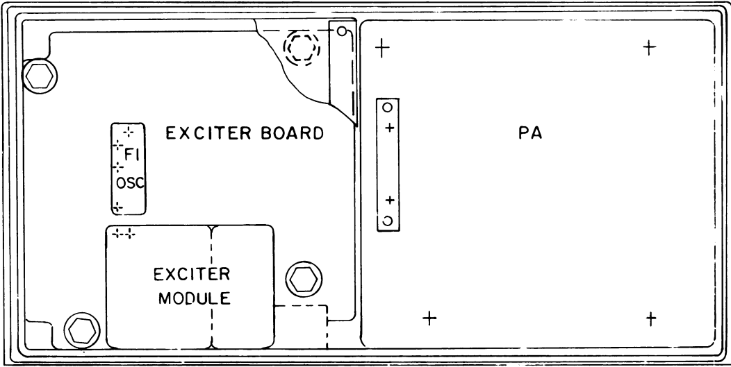
REAR VIEW
