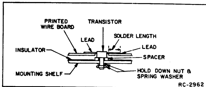
Figure 2 - PA Transistor Q202 Lead Identification and Mounting
