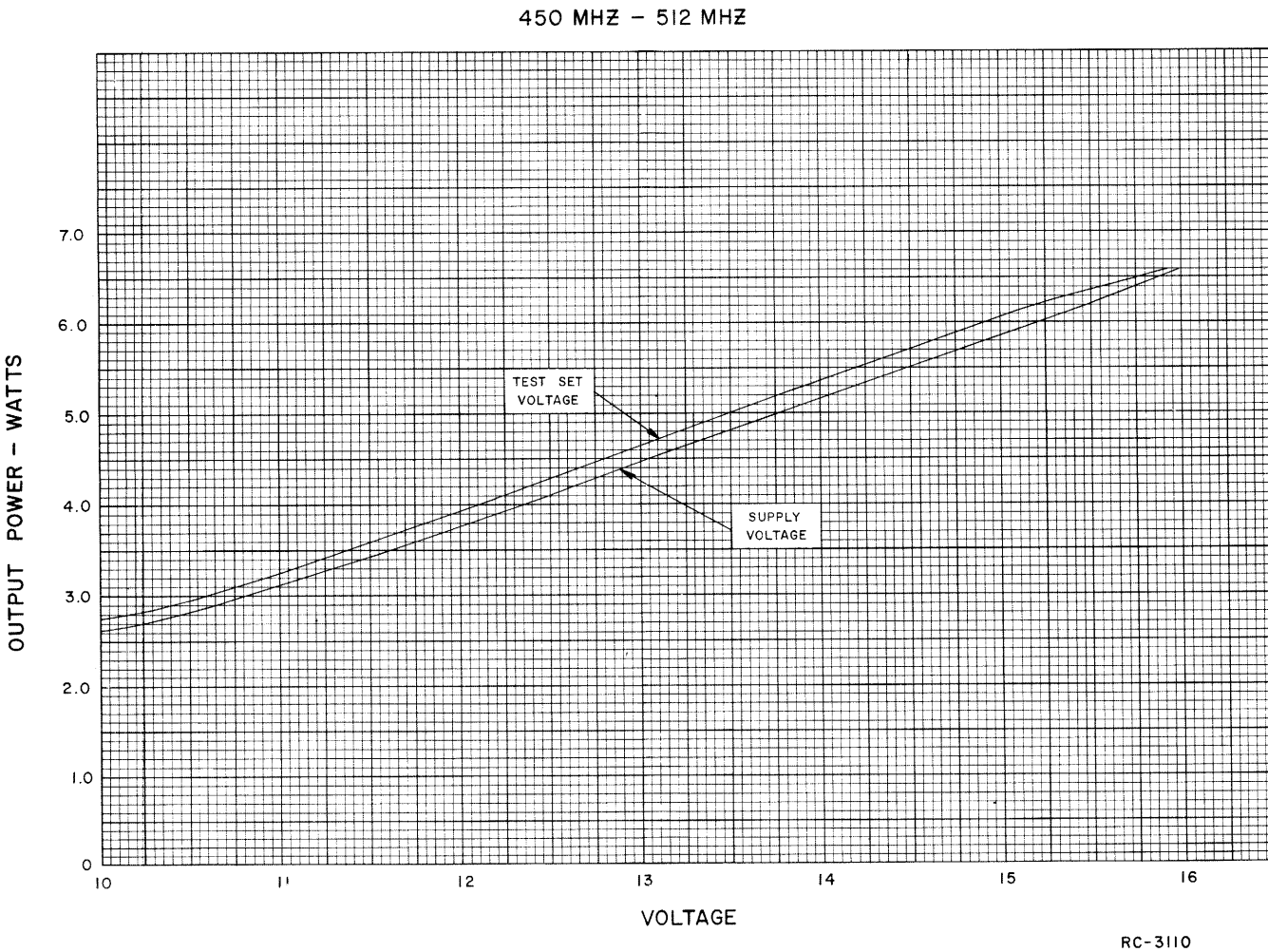
Figure 5 - 450-512 MHz Power Output Setting Chart
