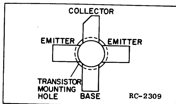
Figure 2 - PA Transistor Q202 Lead Identification and Mounting
