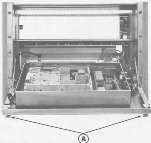
Figure 4 - Access to Exciter Front View
