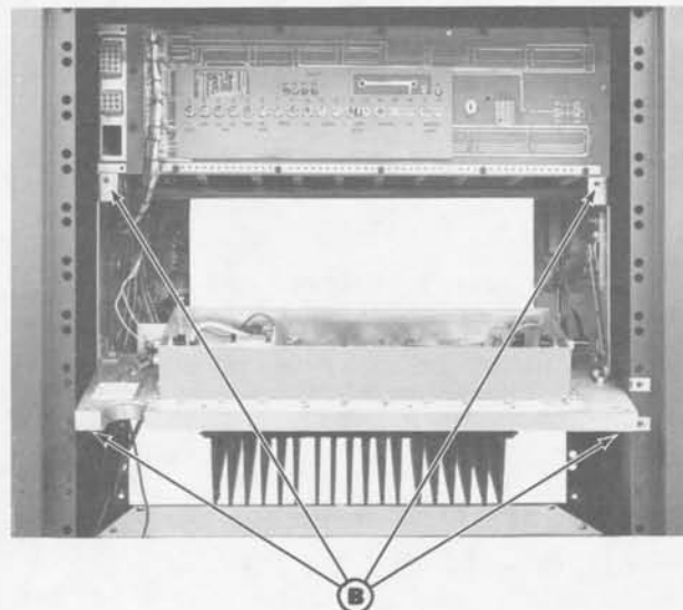
Figure 5 - Access to Power Amplifier Rear View
