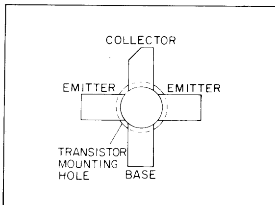
Figure 6 - Lead Identification
