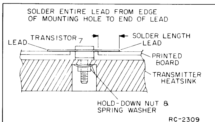
Figure 7 - Lead Forming
