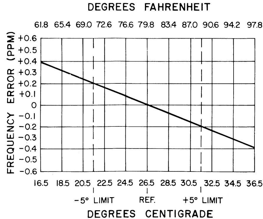
Figure 8 - Frequency Characteristics Vs. Temperature
