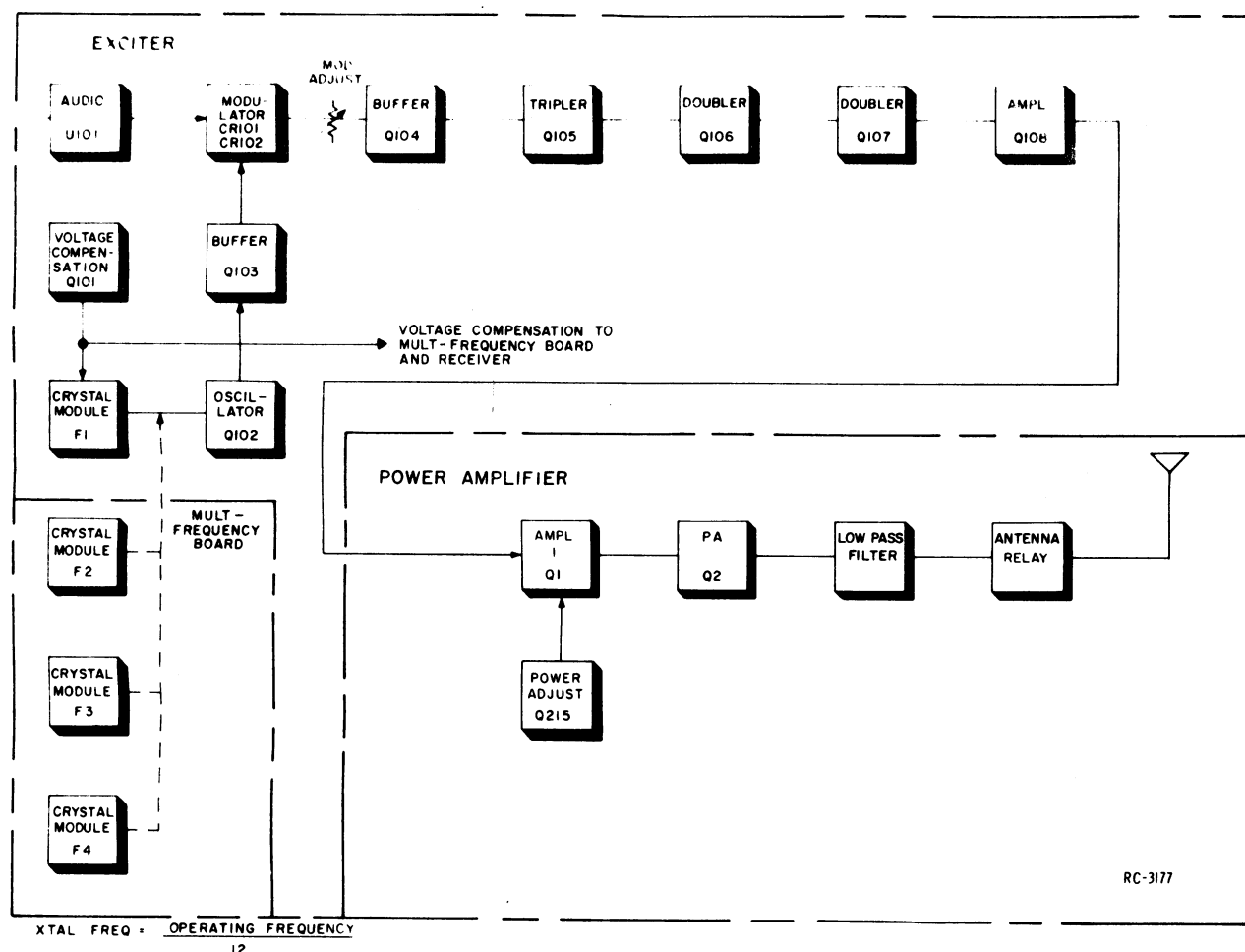
Figure 1 - Transmitter Block Diagram
