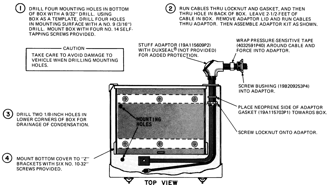
Figure 1 - Installation of Weatherproof Box and Adaptor Kit
