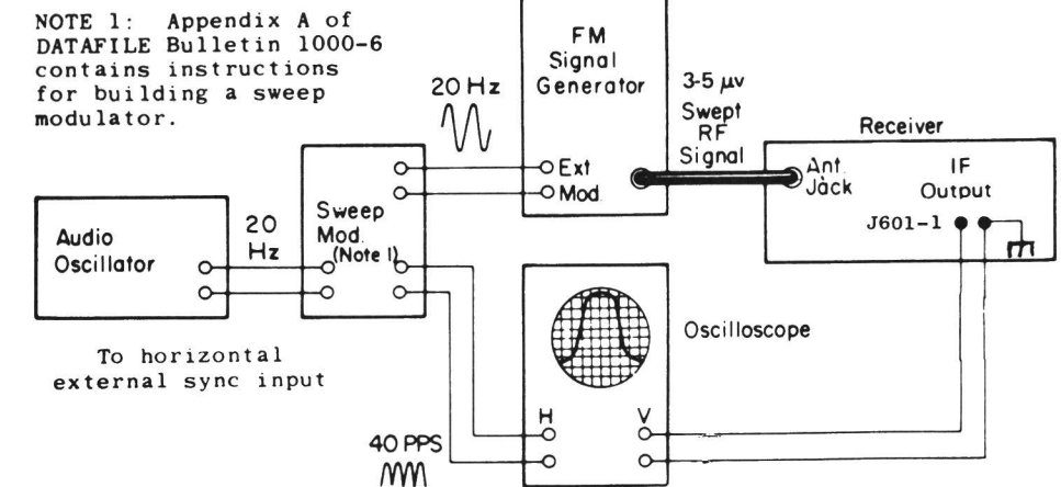
Figure 2 - Test Setup for 20-Hz Double-Trace Sweep Alignment
