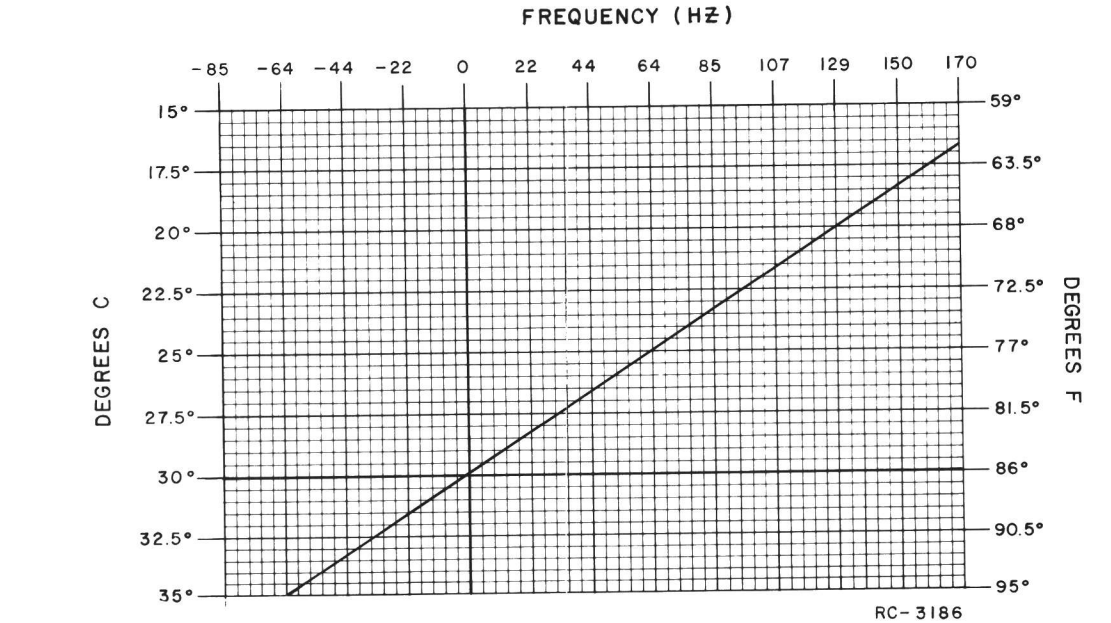
Figure 3 - Frequency Offset Chart
