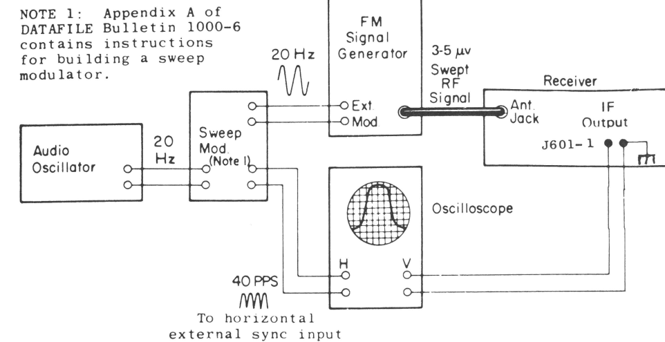
Figure 2 - Test Setup for 20-Hz Double-Trace Sweep Alignment
