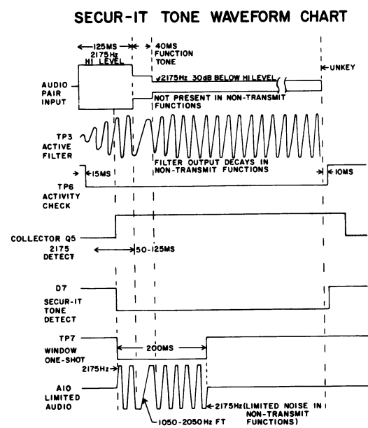
Figure 2 - Tone Control System Troubleshooting
