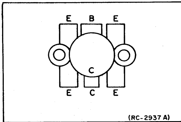
Figure 6 - Lead Identification
