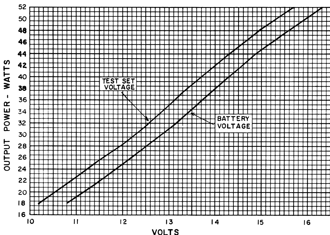
Figure 6 - Power Output Setting Chart
