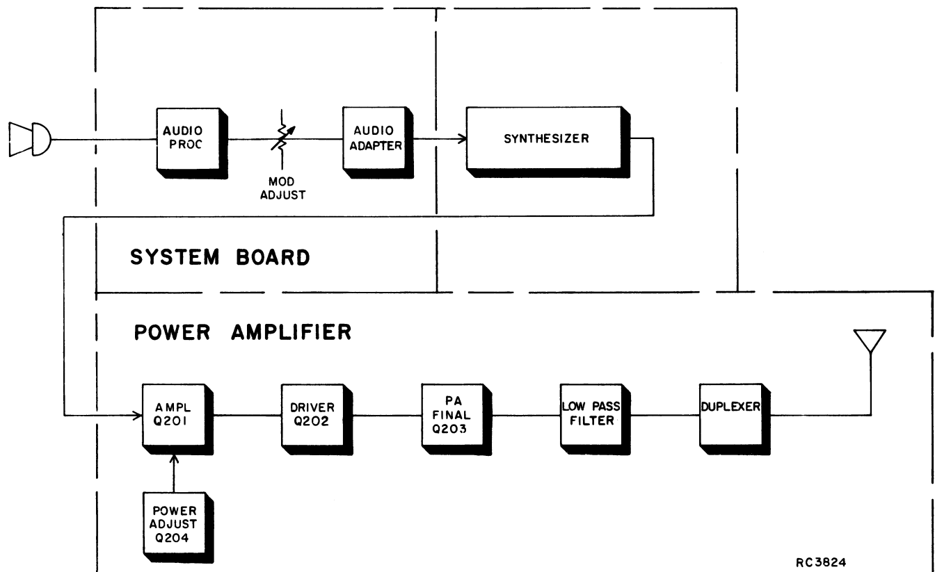
Figure 1 - Synthesized Transmitter Block Diagram
