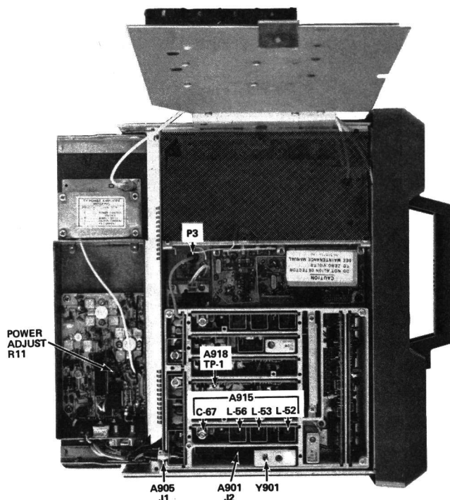
Figure 5 - Alignment Adjustment Location
