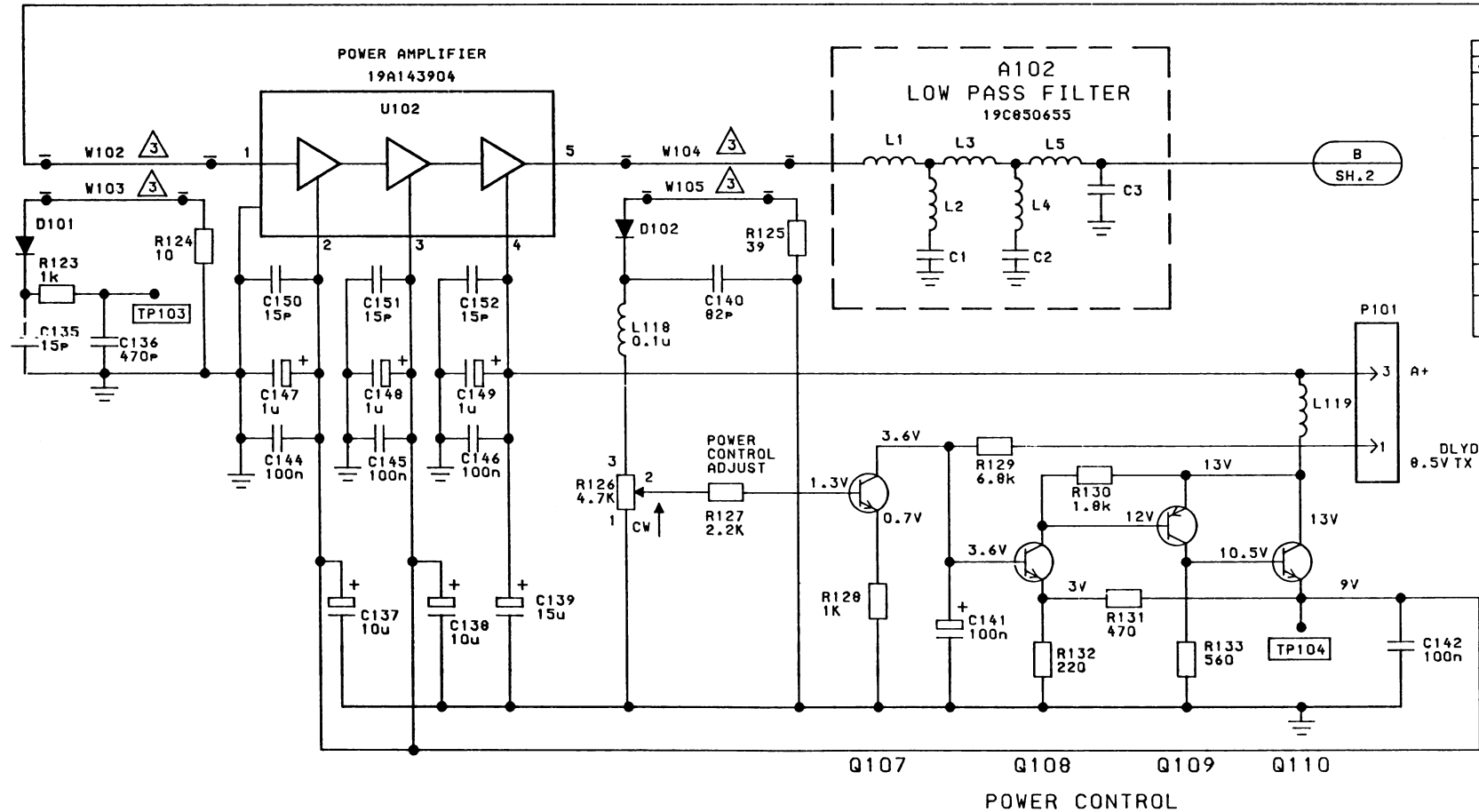
SCHEMATIC DIAGRAM TRANSMITTER
