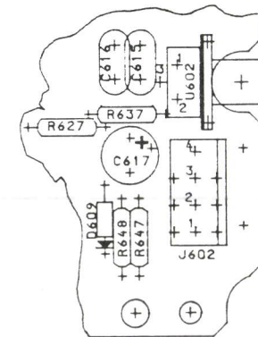
GROUP 3,6 ONLY DETAIL B
