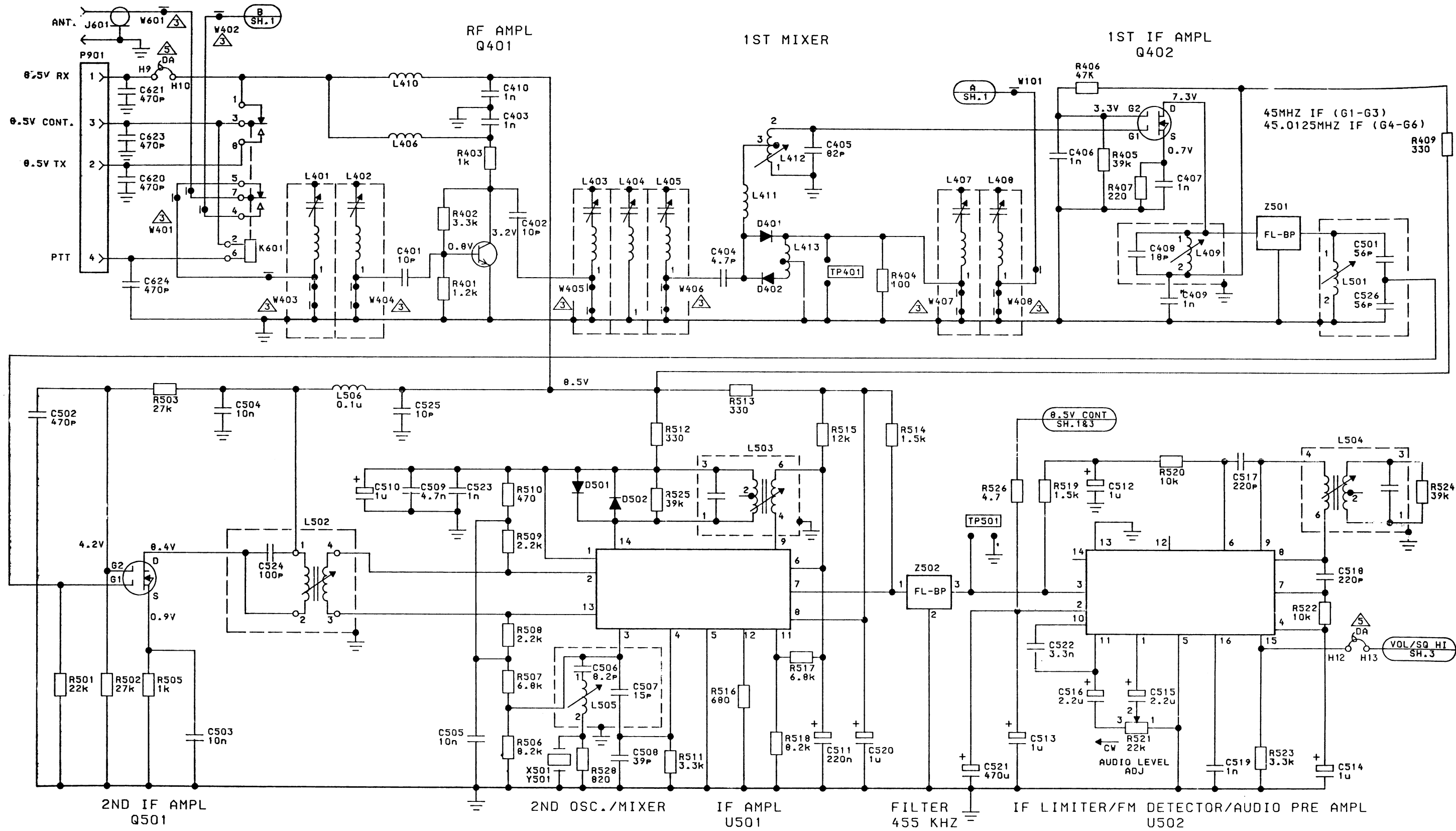
SCHEMATIC DIAGRAM RECEIVER
