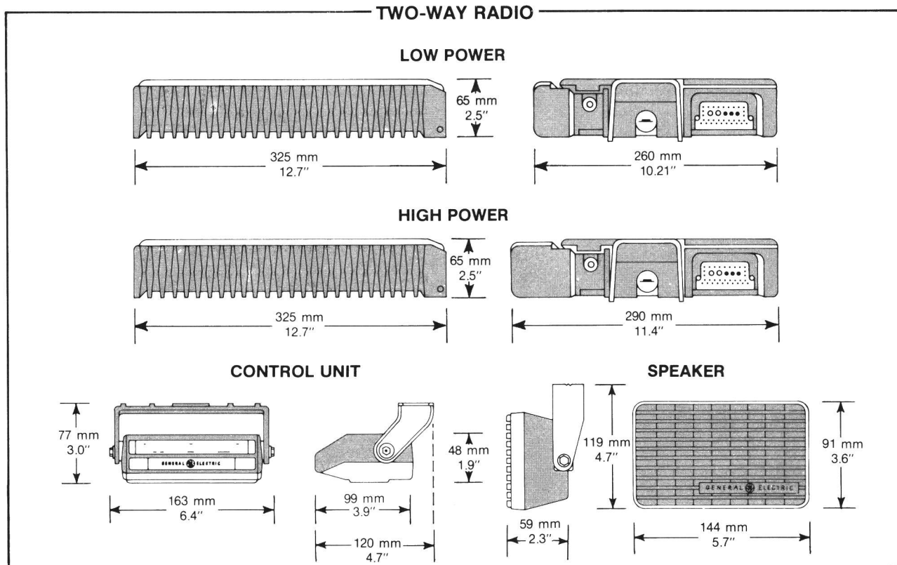
Figure 1. Mounting Dimensions
