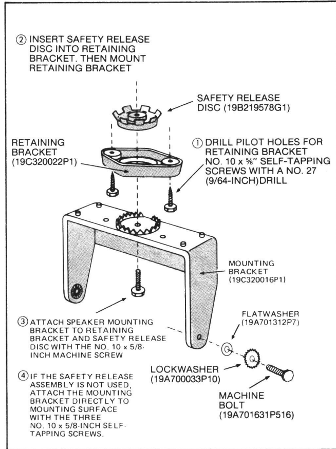
Figure 18. Mounting the Speaker
