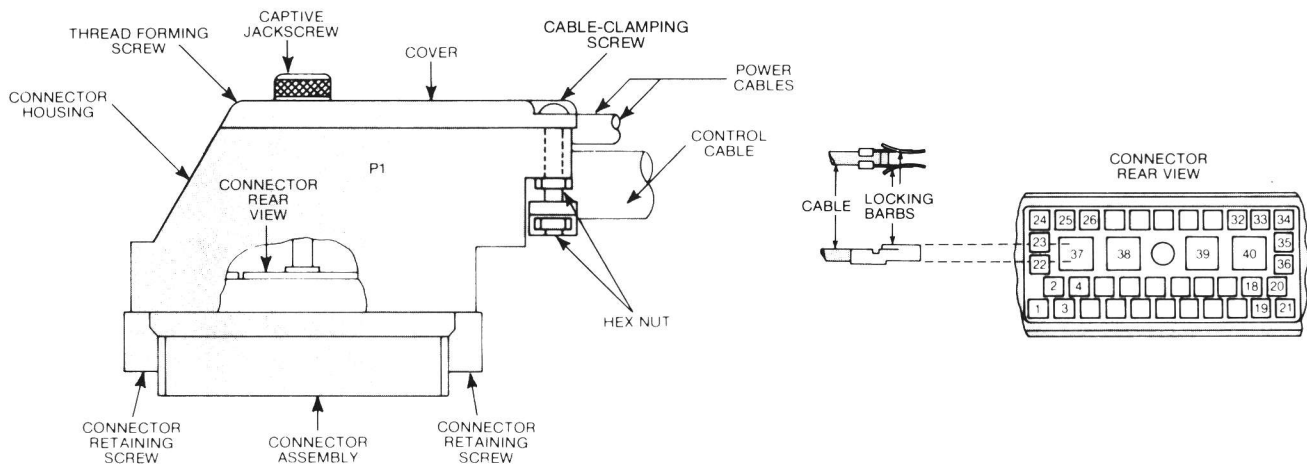
Figure 3. Connector Housing & Terminal Identification
