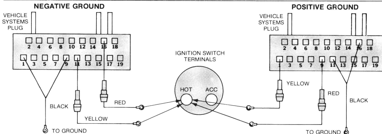
Figure 13. Connections for 12-Volt Ignition Switch Cables
