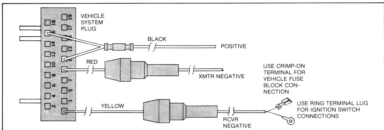
Figure 12. 12-Volt, Positive Ground Connections
