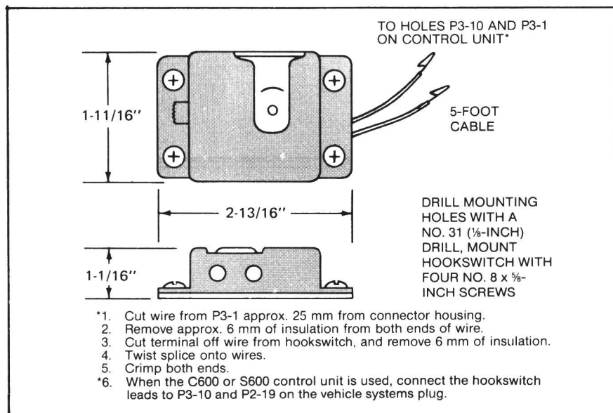
Figure 19. Hookswitch Mounting
