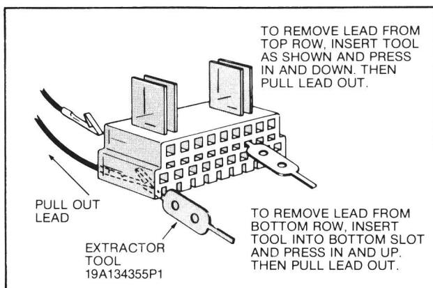
Figure 4. Using Extraction Tool
