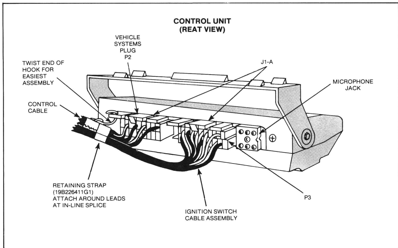
Figure 16. Installing Retaining Strap (S500-S600 Typical)
