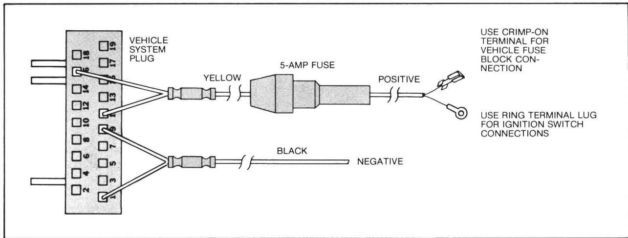
Figure 8. 12-Volt, Negative Ground Connections
