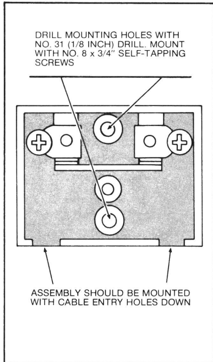
Figure 6. Installation of 12-Volt Fuse Assembly
