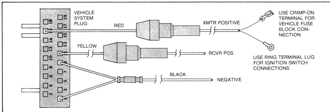
Figure 11. 12-Volt, Negative Ground Connections
