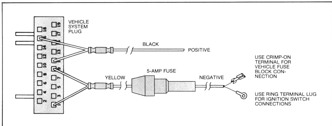
Figure 9. 12-Volt, Positive Ground Connections
