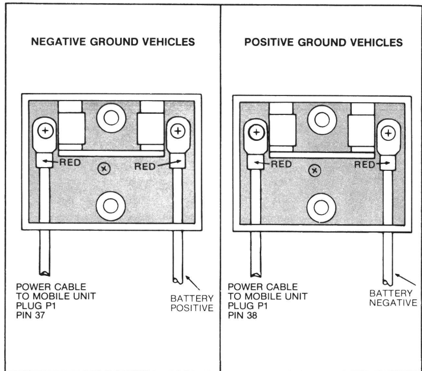
Figure 7. Power Cable Connections to Fuse Assembly
