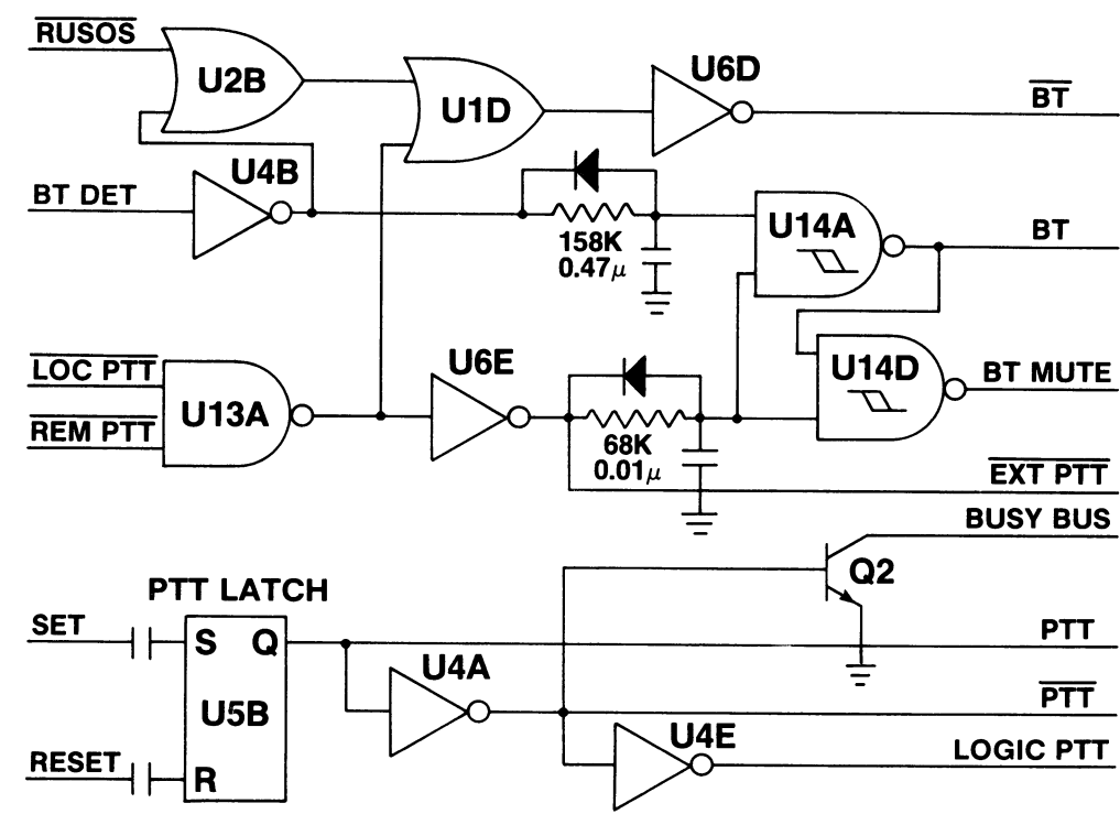
FIGURE 2 DERIVED LOGIC LEADS. RUSOS and BT DET are furnished from the Door Assembly; LOC PTT and REM PTT (test microphone and test switch) come from 10V REG/CNTL BOARD (Control Shelf). The "output" leads shown are all derived in the Repeater Control Board. The first four (BT through EXT PTT) are the direct result of inputs. The remaining four result from the output of PTT LATCH U5B.
