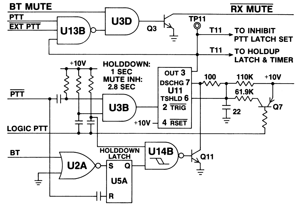
FIGURE 4 MUTE FUNCTION; HOLDDOWN/MUTE INHIBIT TIMER. The RX MUTE output (to IFAS) silences high-level audio and inhibits RUS output with many control consequences. When running, T11 inhibits RX MUTE (Q3 is off via U13B and U3D). Timeout of T11 is inhibited when Q11 is on. T11 times 2.8 seconds when Q7 is off; 1.0 second when Q7 is on.
