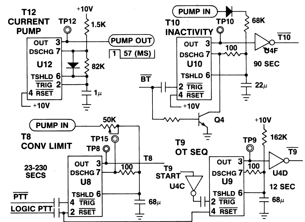
FIGURE 3 TIMERS T8, T9, T10 AND T12. All use "555" timers. T12, astable connected, delivers charging current to T8 and T10. Duty factor is 1/58; RC-determined timed periods are multiplied. T8, T9 and T10 start with logic inputs; T8 and T9 reset with logic inputs. Timeout of T10 is inhibited when Q4 is on. Outputs go to circuits which reset PTT Latch U5B (XMTR OFF). All timers have an output Test Point (1=running or inhibited; 0=reset).
