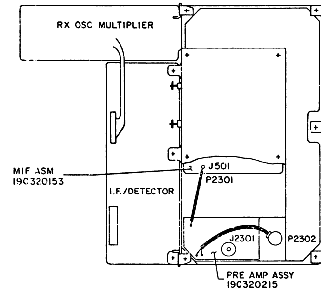
NOISE BLANKER-PRE AMP HIGH BAND
