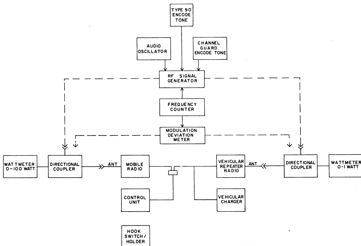
Figure 4 - Test Setup
