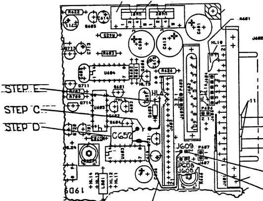
DELTA S/SX SYSTEM BD. AFTER MODIFICATION
