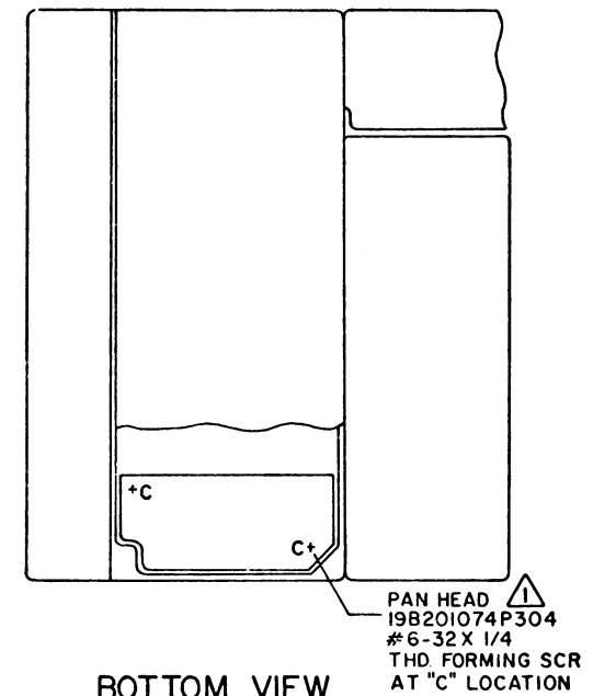
NOISE BLANKER-PRE AMP HIGH BAND
