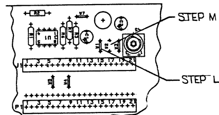
19D900561 MII INTERFACE BD. COMPONENT SIDE
