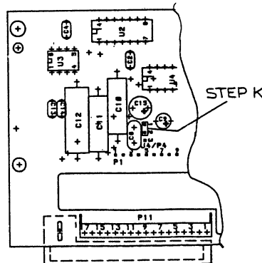
19D901775 CHANNEL GUARD BD. COMPONENT SIDE
