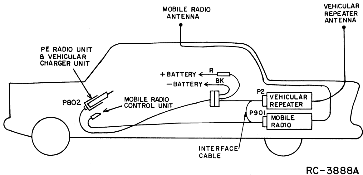
Figure 3 - Typical Installation in Vehicle
