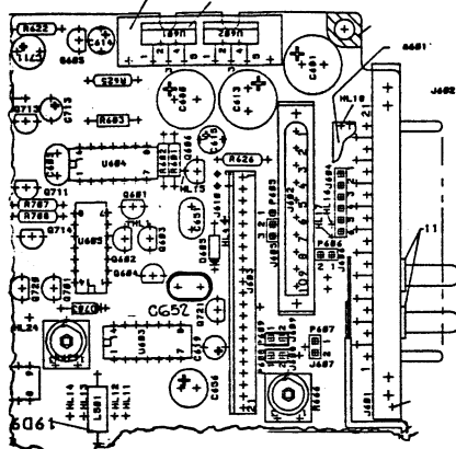
DELTA S/SX SYSTEM BD. BEFORE MODIFICATION
