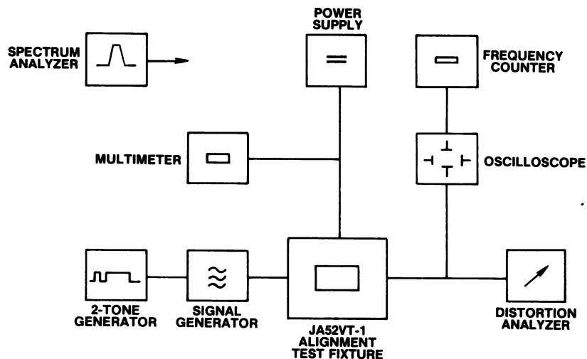
Figure 6 - Alignment Setup
