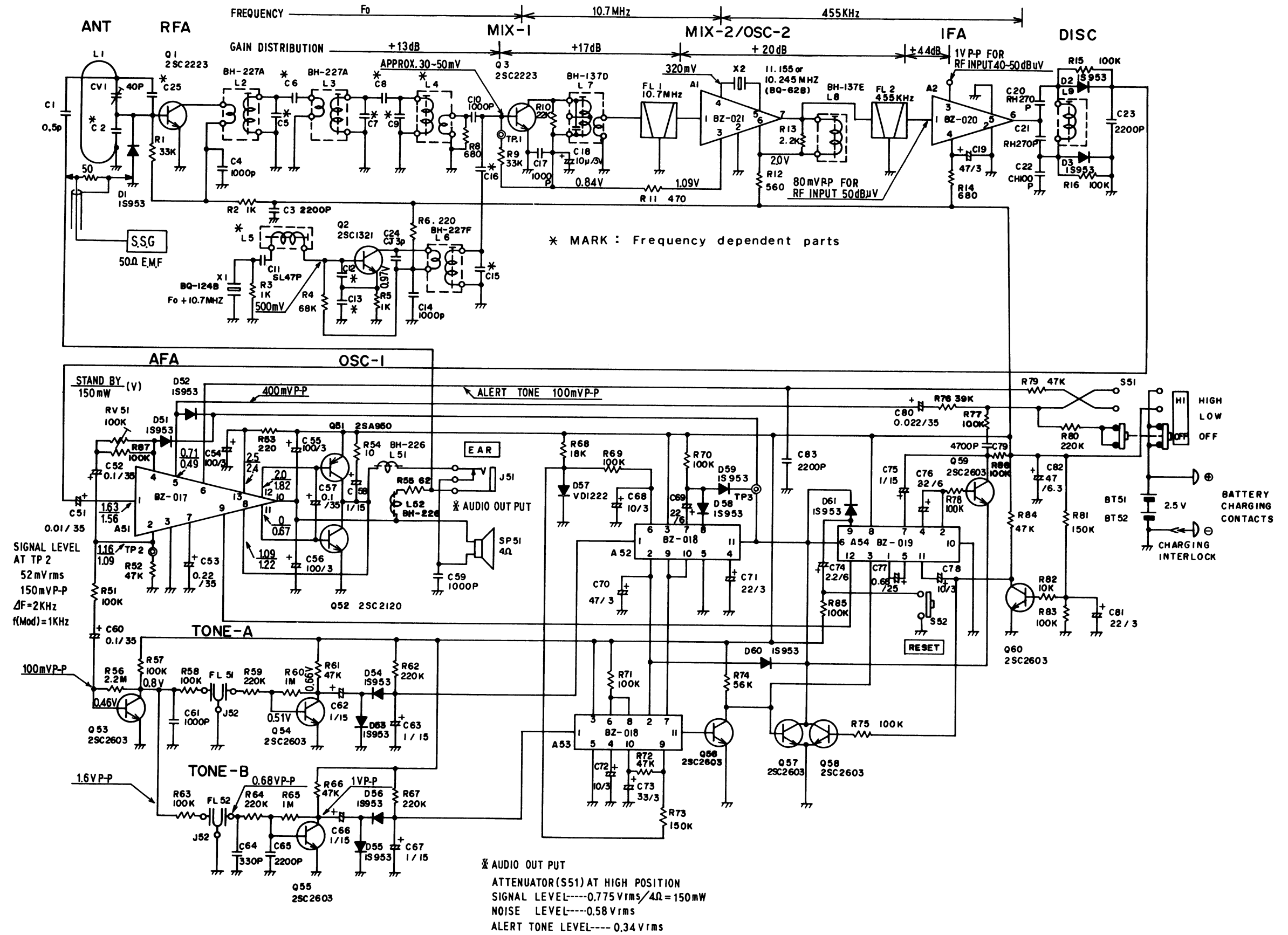
SCHEMATIC DIAGRAM
