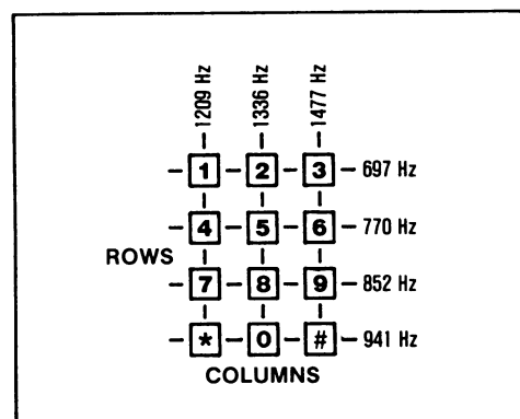
Figure 1 - Touch-Tone Keypad and Frequency Format
