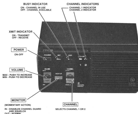
Figure 2 - Standard Two Channel Radio
