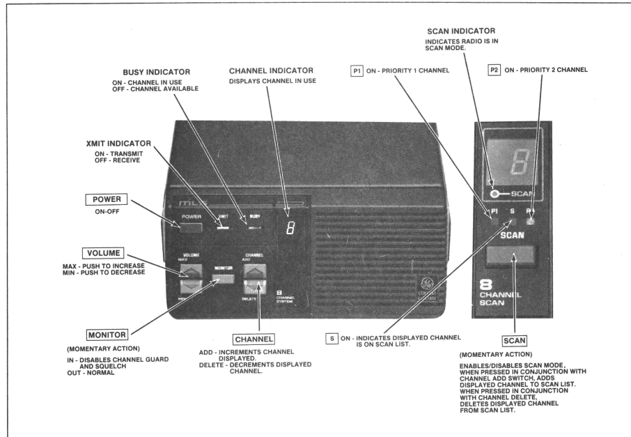
Figure 3 - Eight Channel Radio Without Scan/With Scan
