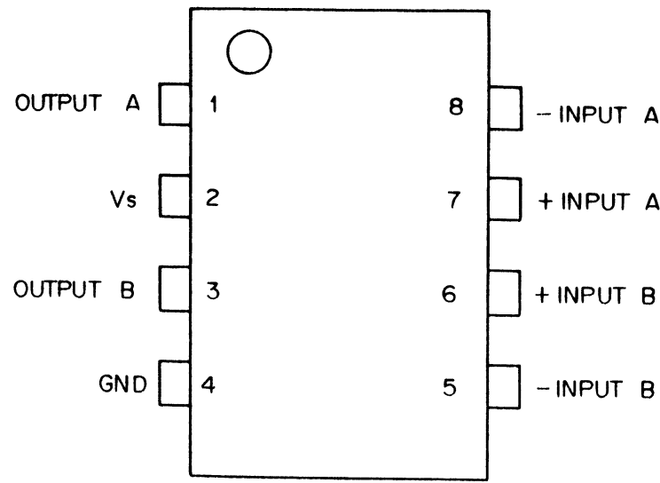
Pin Arrangment
