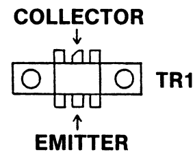
Figure 2 - PA Transistor Lead Identification
