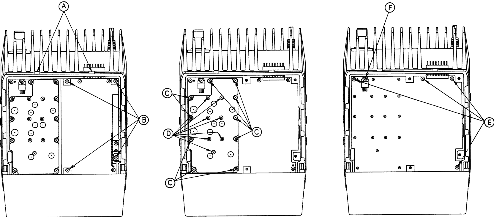
Figure 3—Disassembly Procedure (Top View)
