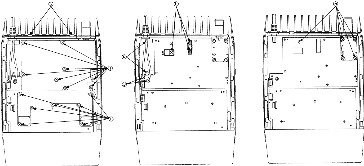
Figure 4—Disassembly (Bottom View)
