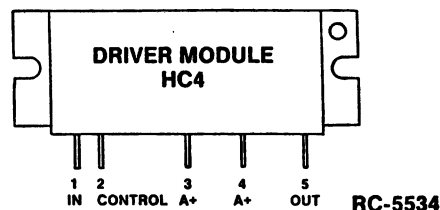
Figure 1 - Driver Lead Identification
