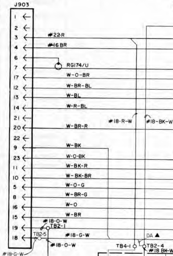
DETAIL "A" FOR UHF SYSTEMS
