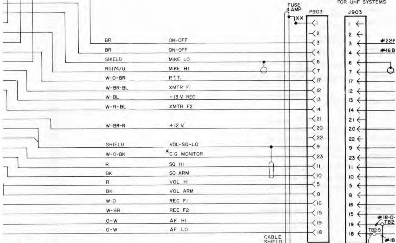
DETAIL "A" FOR UHF SYSTEMS
