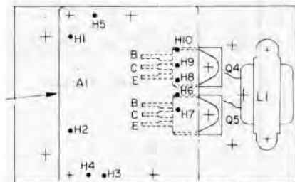
10-WATT AUDIO AMPLIFIER (USED WITH 24/36 V POWER SUPPLY)
