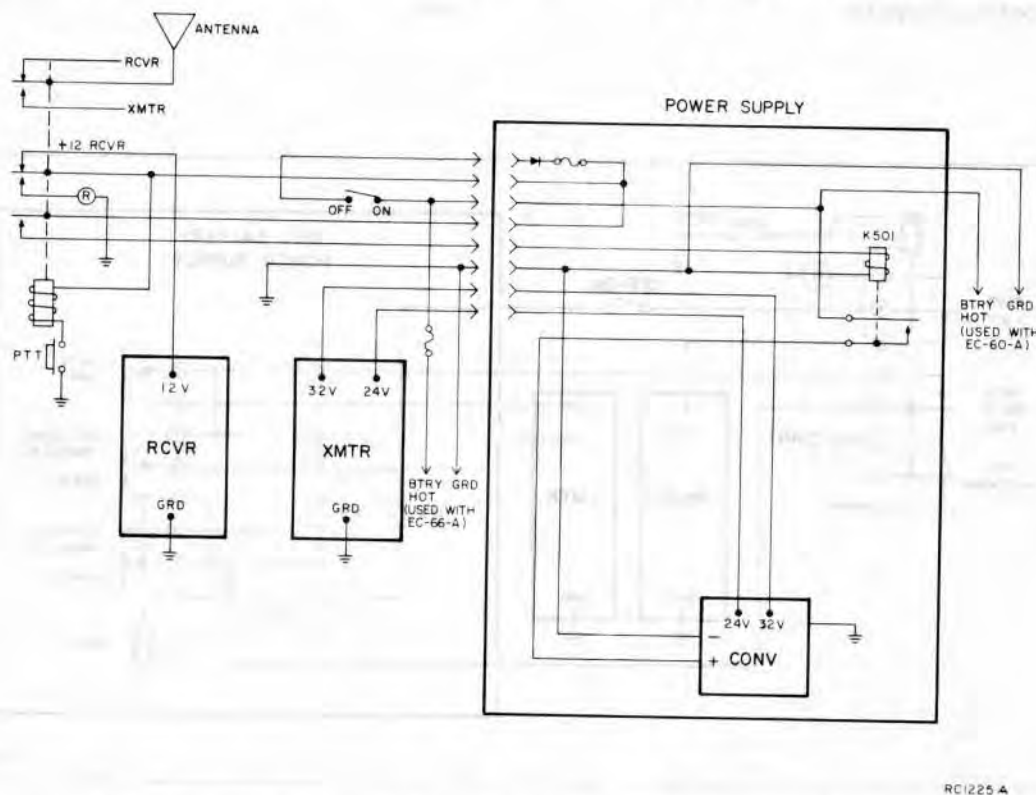
Figure 6 - Antenna Switching and Power Distribution for Model 4EP47A11
