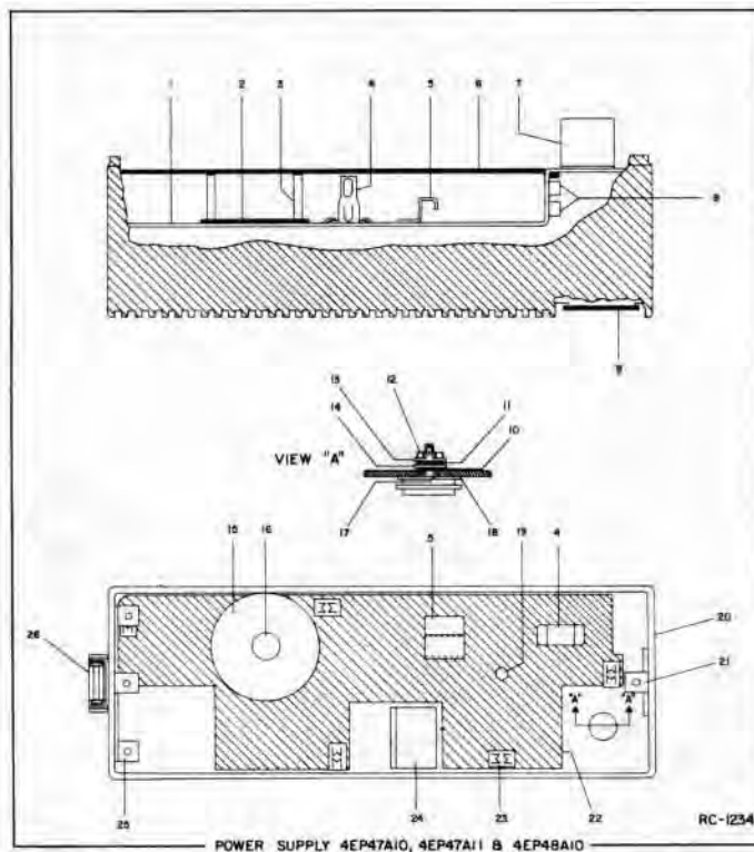
POWER SUPPLY 4EP47A10, 4EP47A11 B 4EP48A10
