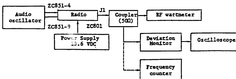
Measuring system
