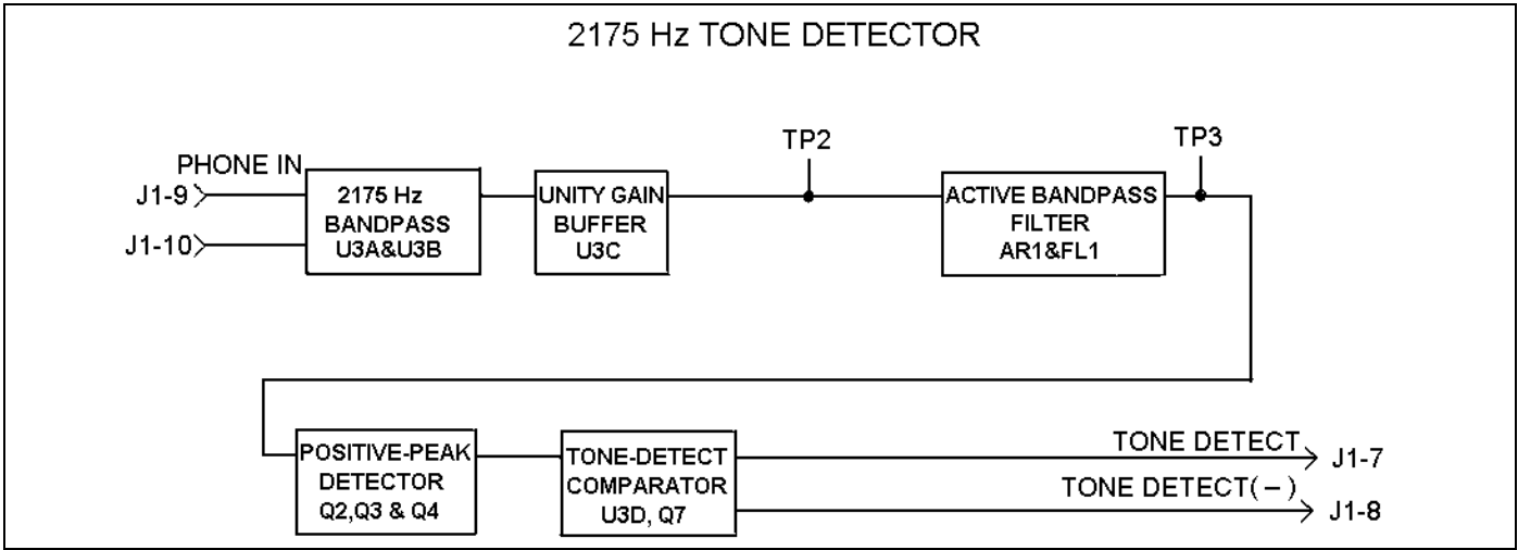
Figure 1 - Console Interface Board Block Diagram
