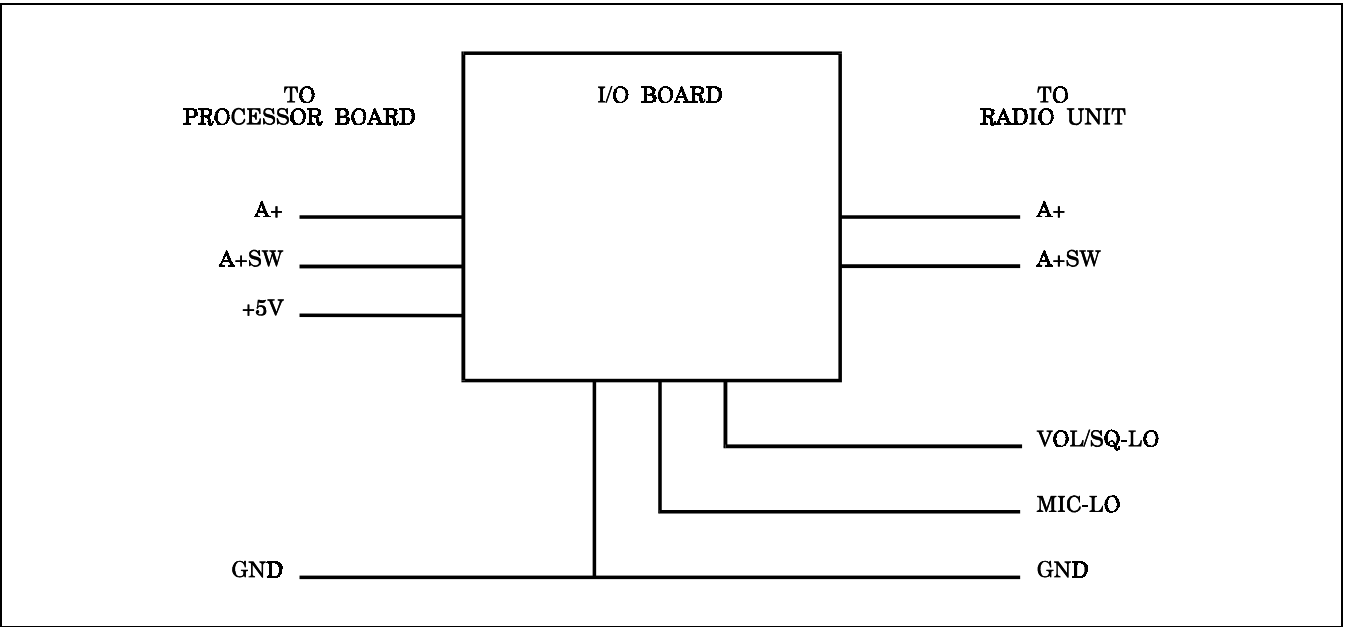
Figure 1 - I/O Board Power Distribution
