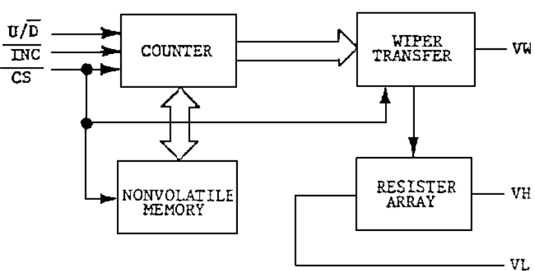
FUNCTIONAL DIAGRAM
