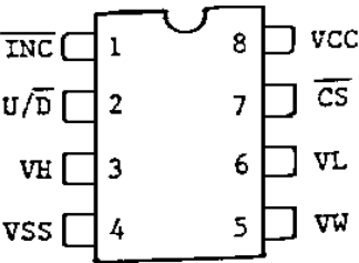
PIN CONFIGURATION
