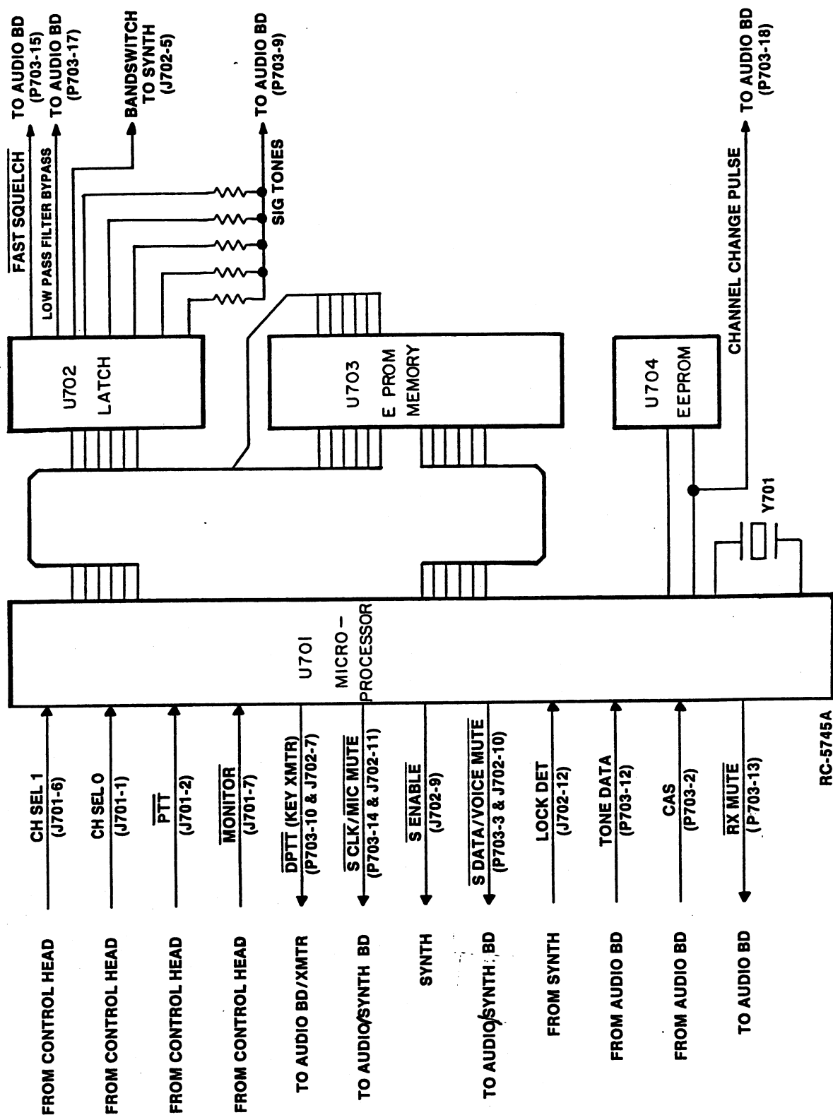
FIGURE 1 - BLOCK DIAGRAM
