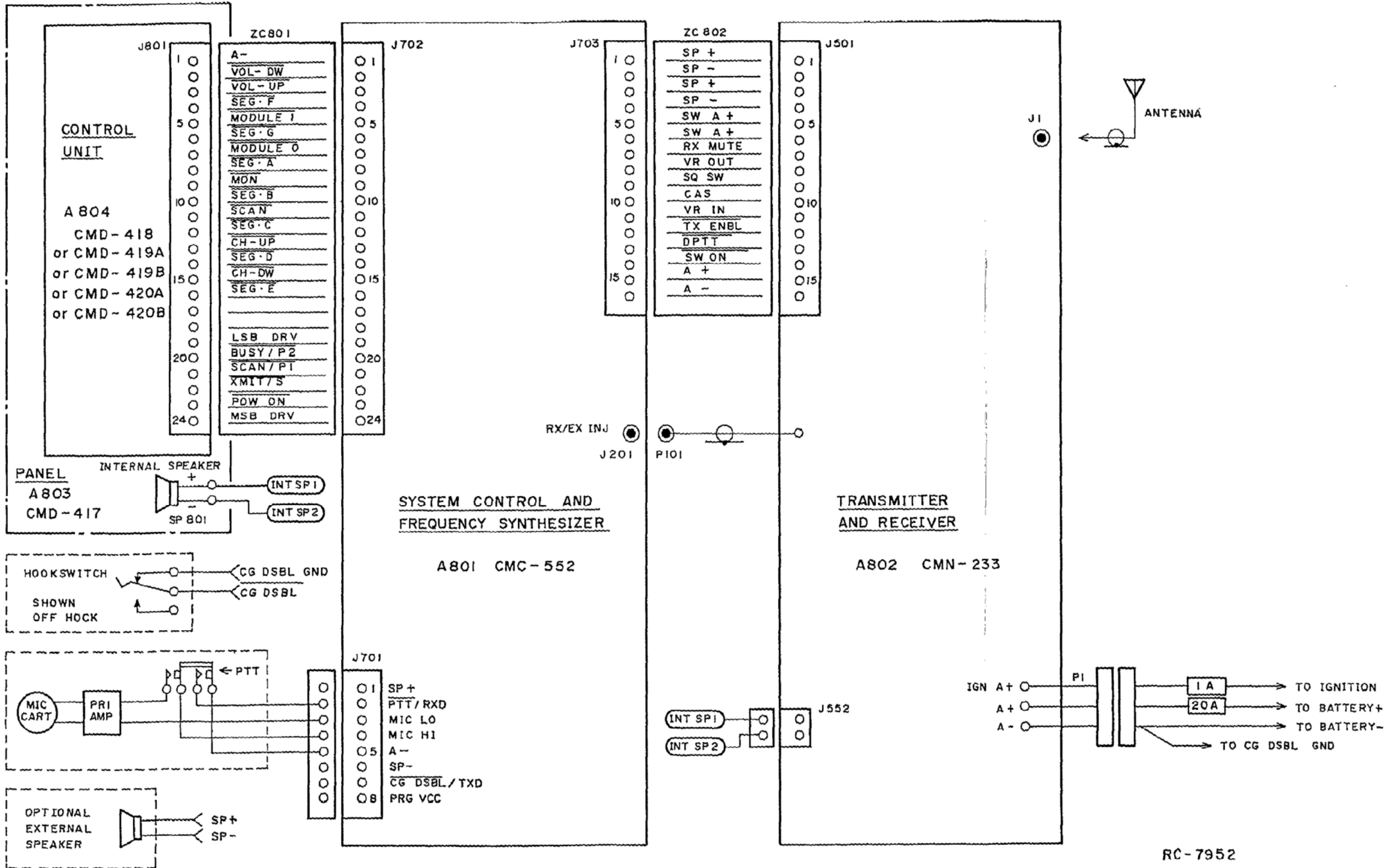
Figure 1 - Interconnection DiagramFigure 2
