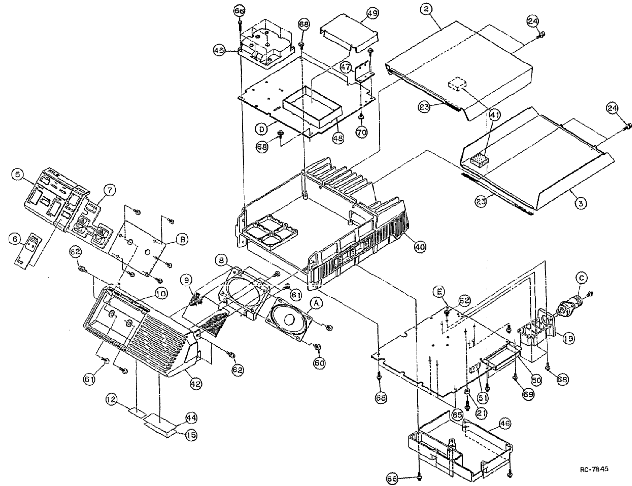
Figure 3 - Mechanical Parts Breakdown
