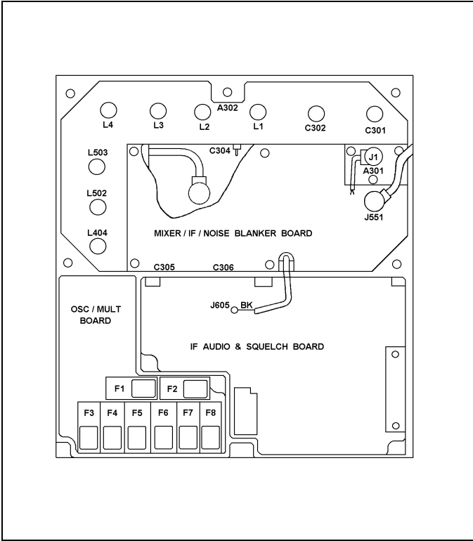
Figure 4 - Receiver Module Location Diagram
