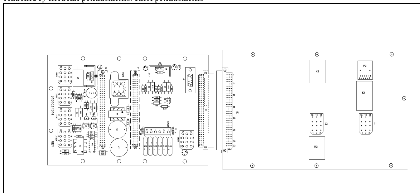
Figure 1 - Backplane and Auxiliary Backplane Boards
