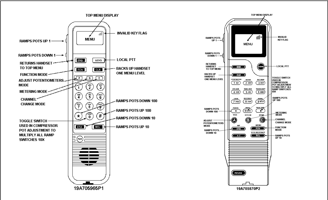
Figure 2 - Handset Operations
