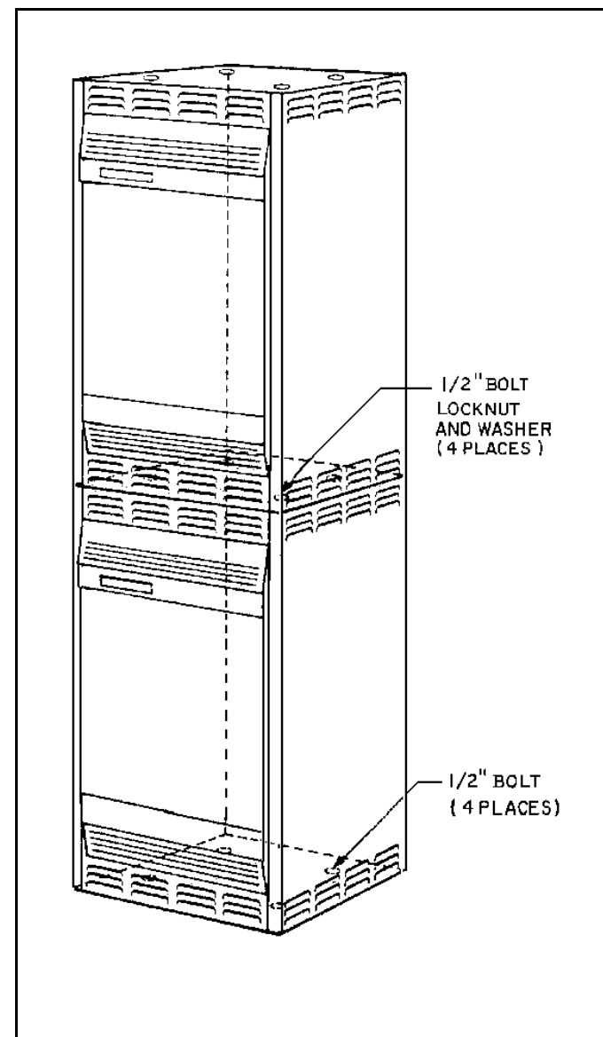
Figure 4 - Stacked 37-Inch Cabinets
