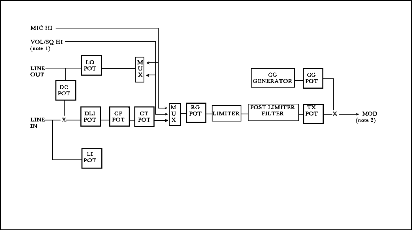
Figure 16 - MASTR III System Module Pot Alignment
