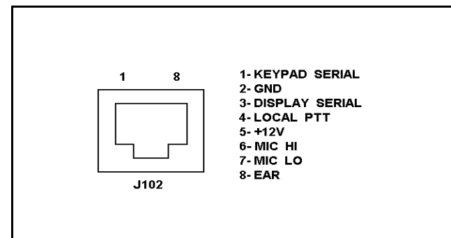
Figure 5 - Microphone Connections
