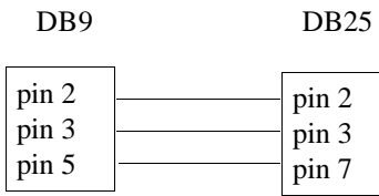
Figure 12 - 3-Wire Adapter
