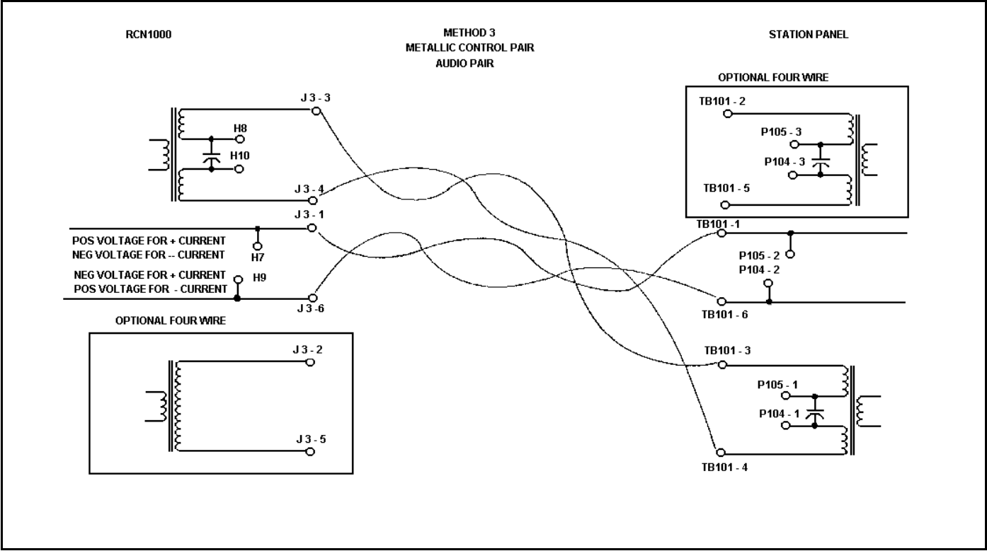
Figure 9 - METHOD 3 (Metallic Control Pair, Audio Pair)
