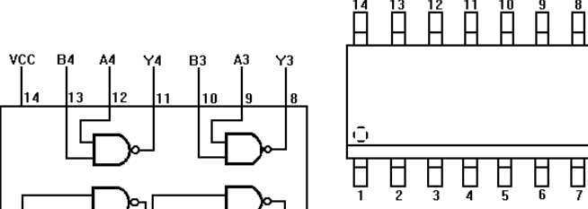
U701 & U705 19A703483P302 Quad 2-Input NAND Gate
