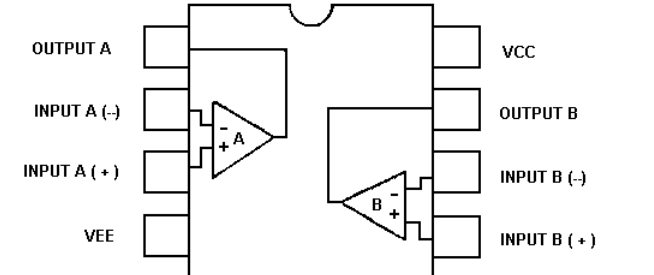
U501 344A3070P1 Operational Amplifier
