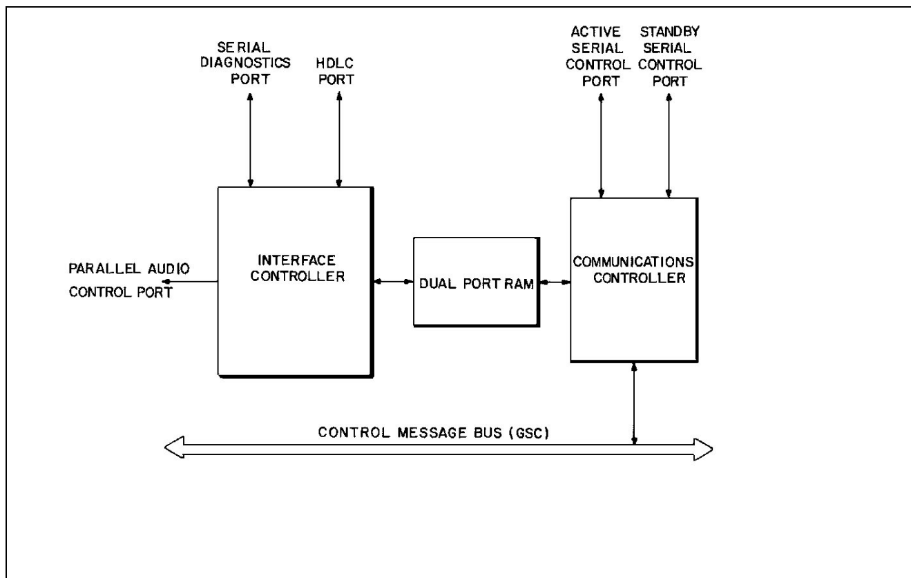
Figure 4 - Controller Board Architecture
