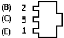
LEAD IDENTIFICATION FOR Q1,Q3,Q8
