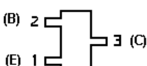
LEAD IDENTIFICATION FOR Q2,Q4,Q7
