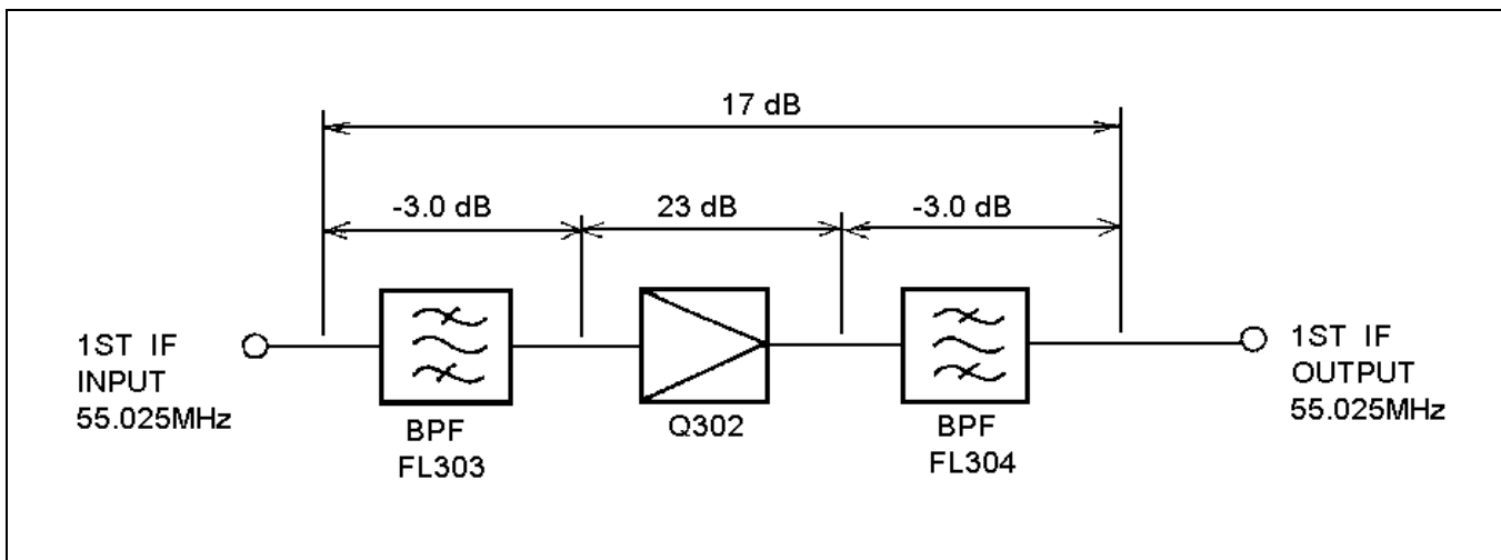
Figure 9 - First IF Amplifier
