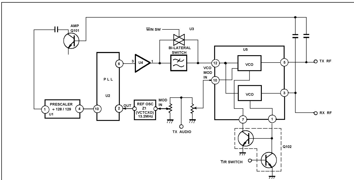
Figure 11 - Synthesizer
