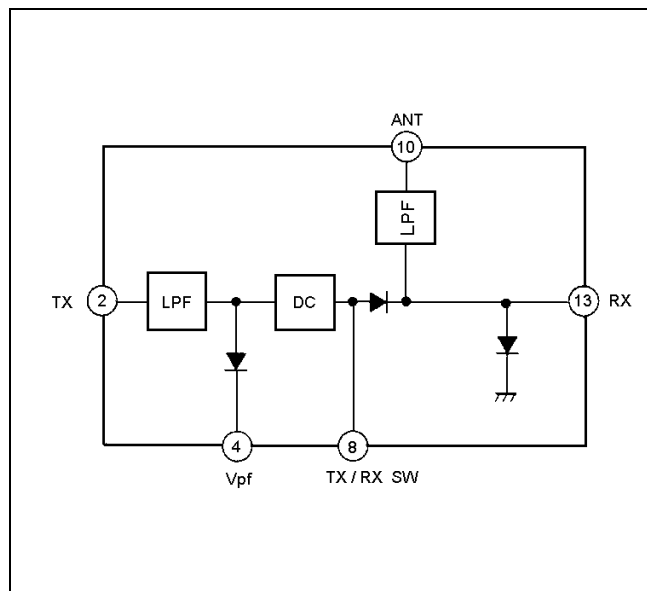
Figure 7 - LPF/DC/T/R SW. Module (U8) VHF/UHF
