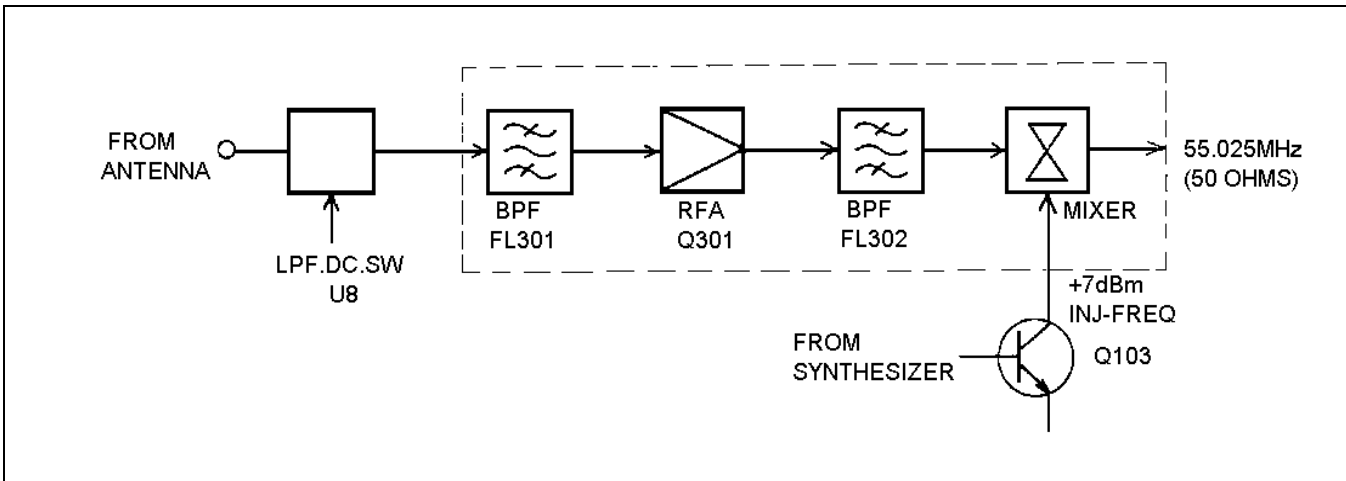
Figure 8 - RF Amplifier/Mixer
