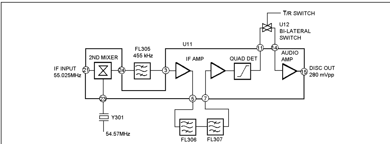
Figure 10 - Second IF Amplifier/Discriminator
