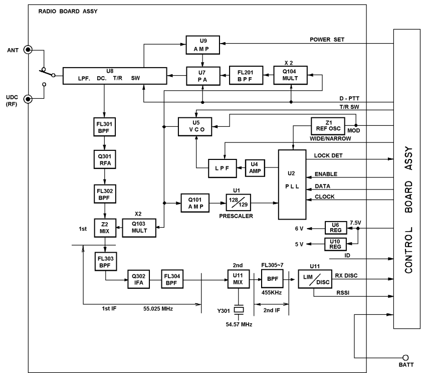
Figure 3 - Radio Block Diagram VHF/UHF
