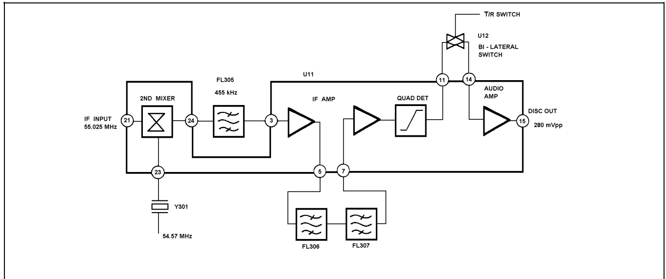
Figure 10 - Second IF Amplifier/Discriminator
