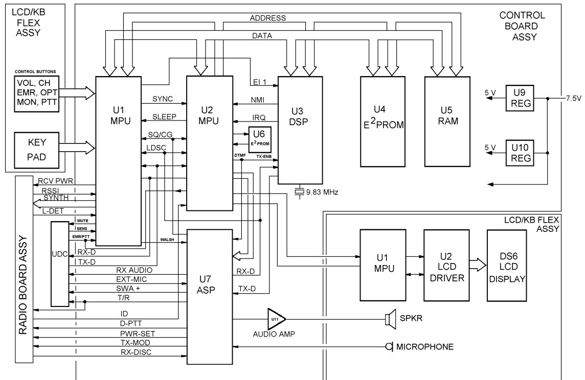
Figure 5 - M-RK II &amp; Scan Logic Block Diagram
