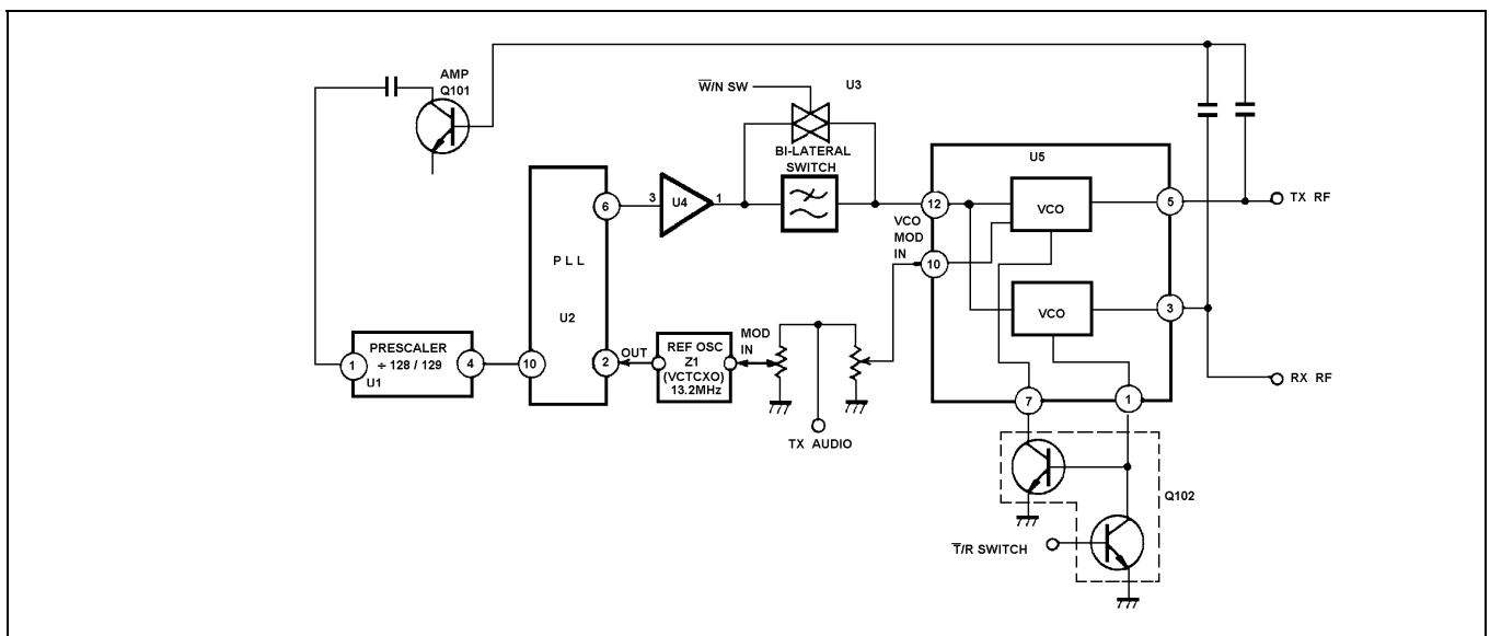
Figure 11 - Synthesizer
