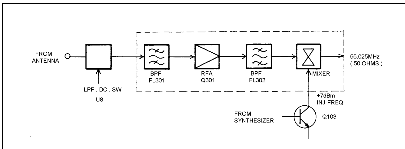
Figure 8 - RF Amplifier/Mixer
