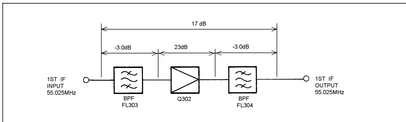
Figure 9 - First IF Amplifier
