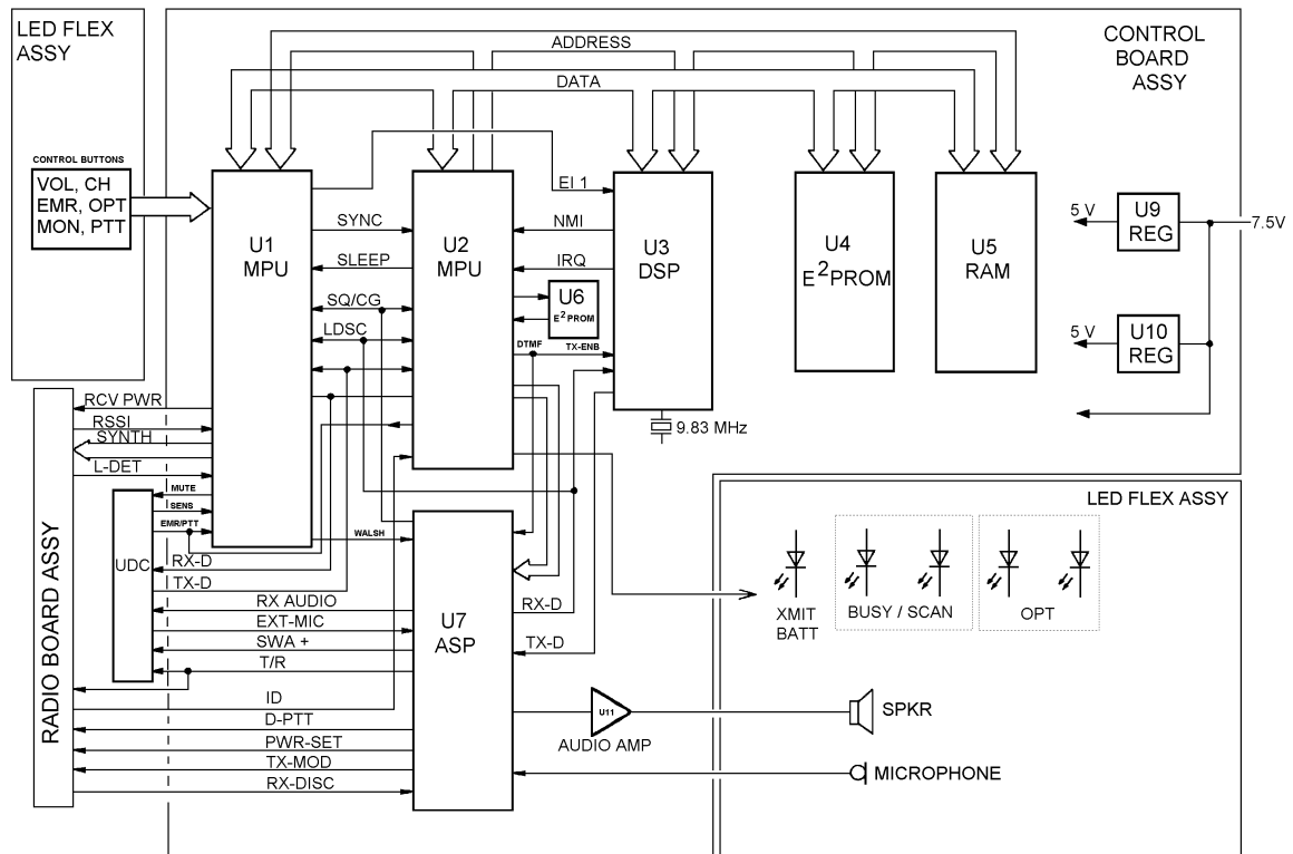
Figure 4 - M-RK I Logic Block Diagram
