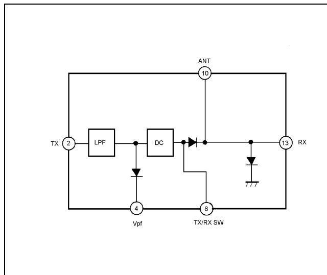
Figure 7 - LPF/ DC/ T/R SW. Module (U8)
