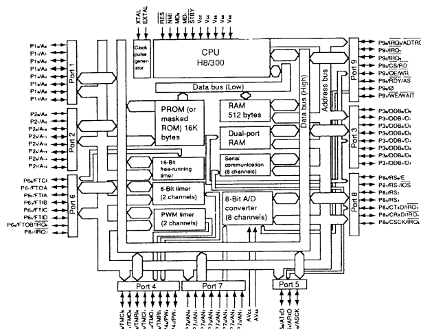
BLOCK DIAGRAM
