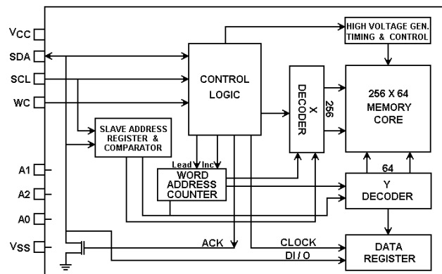
BLOCK DIAGRAM
