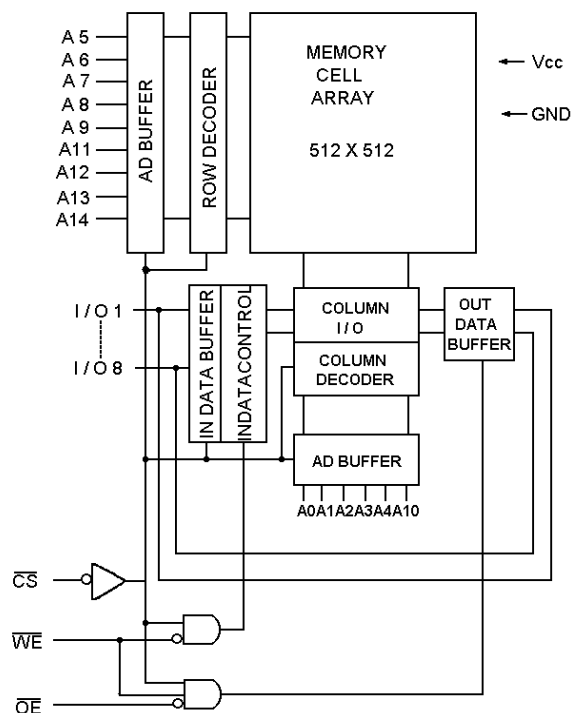
BLOCK DIAGRAM
