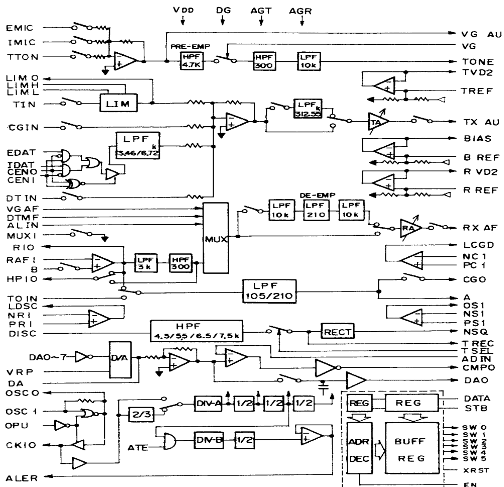
BLOCK DIAGRAM
