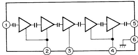
INTERNAL DIAGRAM
