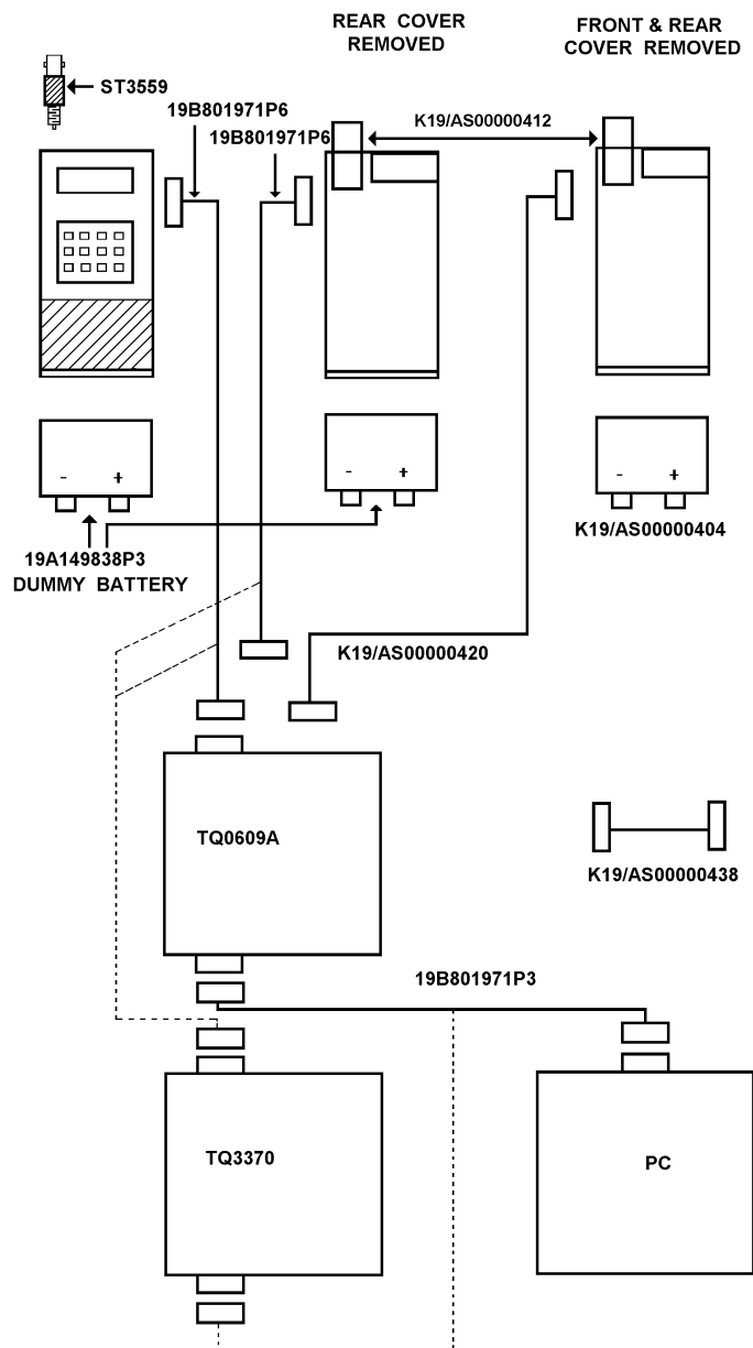
Figure 1A - Servicing Setup
