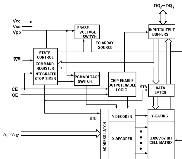
BLOCK DIAGRAM
