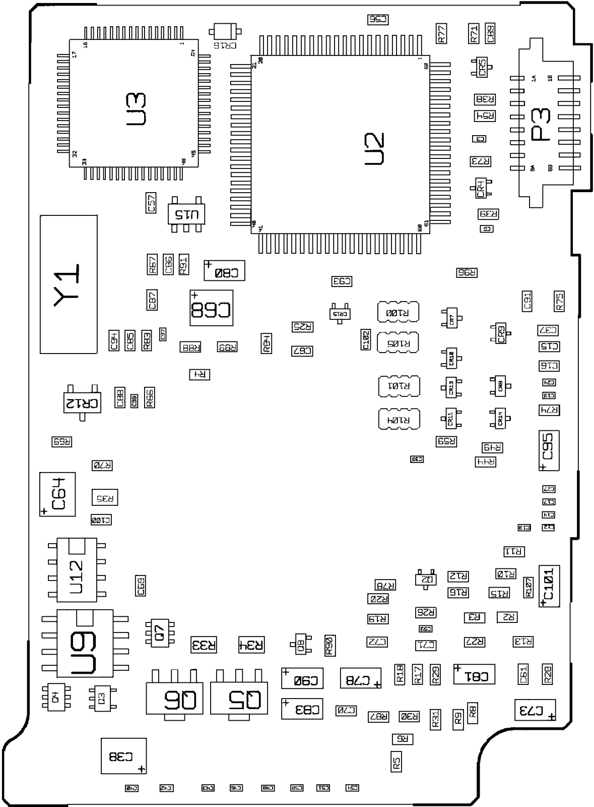
CONTROL BOARD
