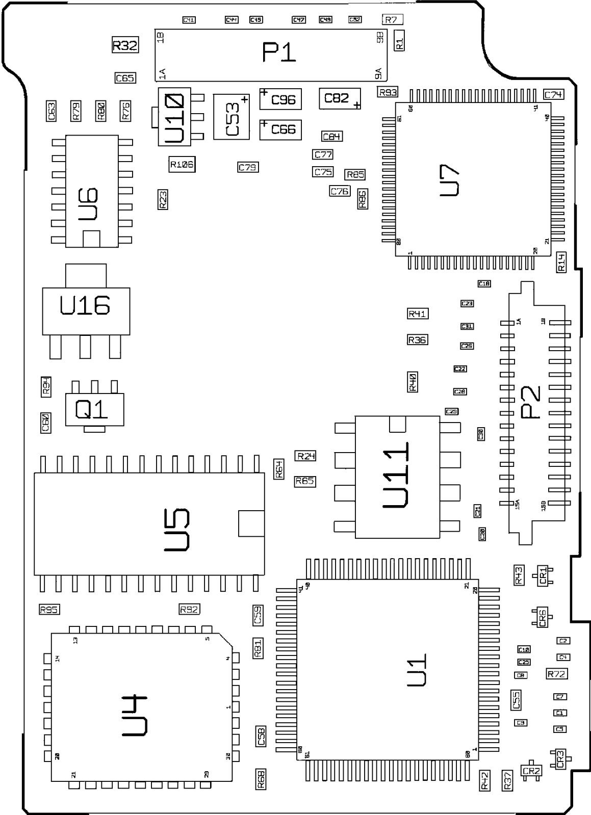
CONTROL BOARD
