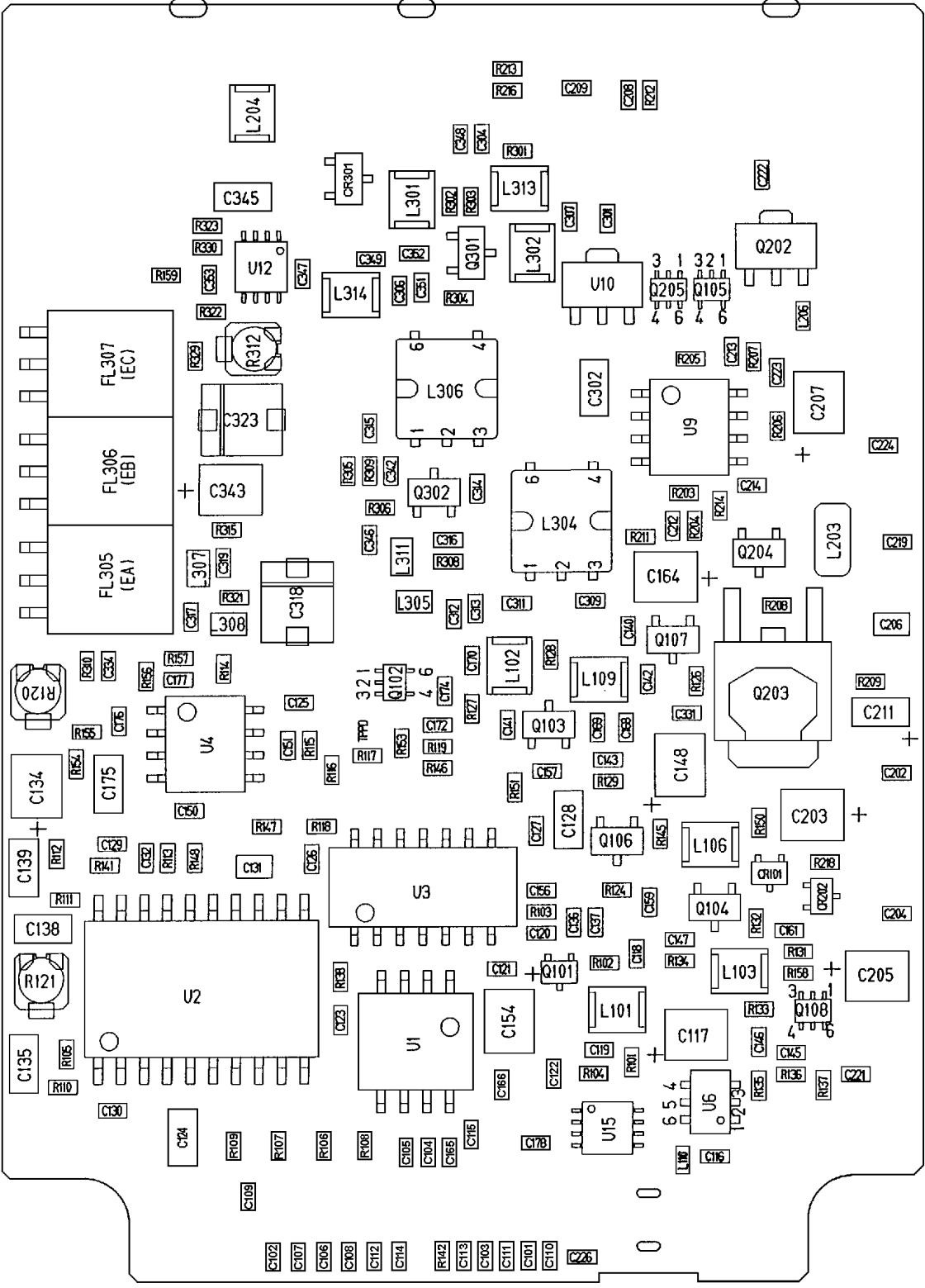
RF BOARD (FCC/DOC/ETS) VHF/UHF SWITCHABLE (A3WE06455, Sh. 1, Rev. 1) (A3WE06455, Sh. 2, Rev. 1)
