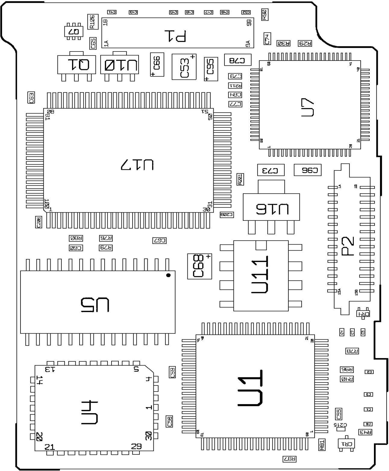
CONTROL BOARD (AEGIS) 256K FLASH
