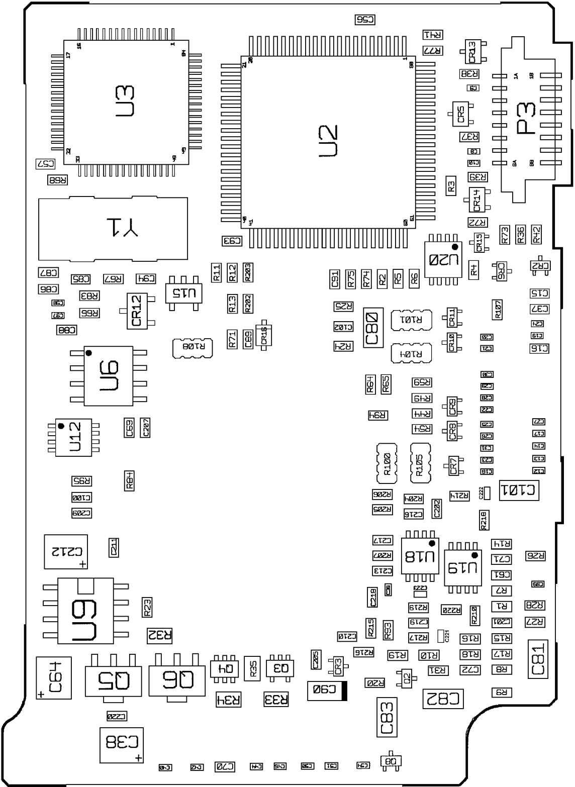
CONTROL BOARD (AEGIS) 512K FLASH
