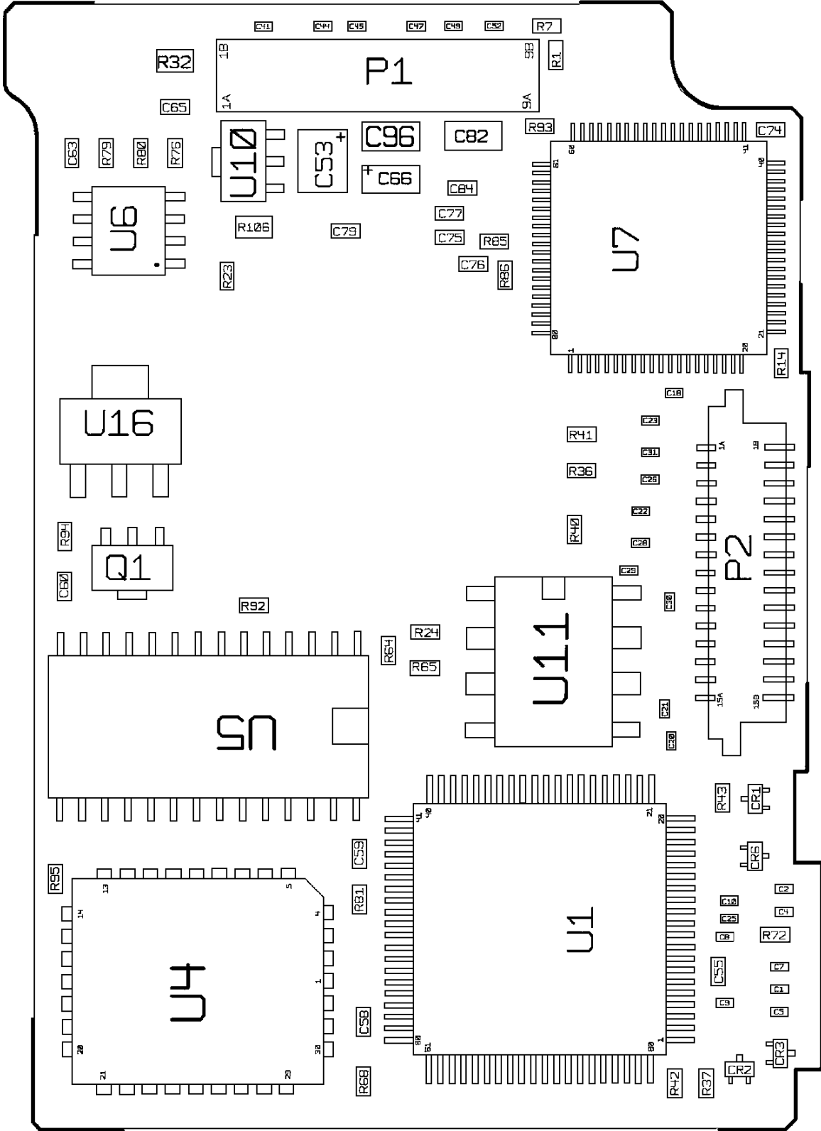
CONTROL BOARD (ANALOG) 512K FLASH
