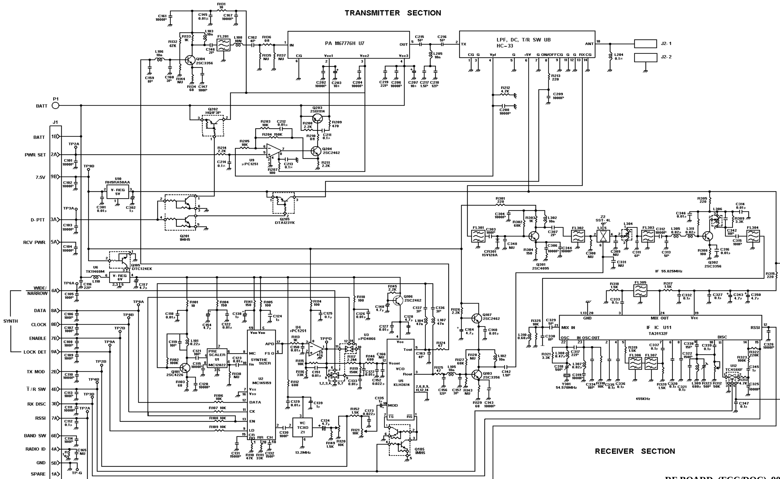
RF BOARD (FCC/DOC) 900 MHz K19/AS00000172
