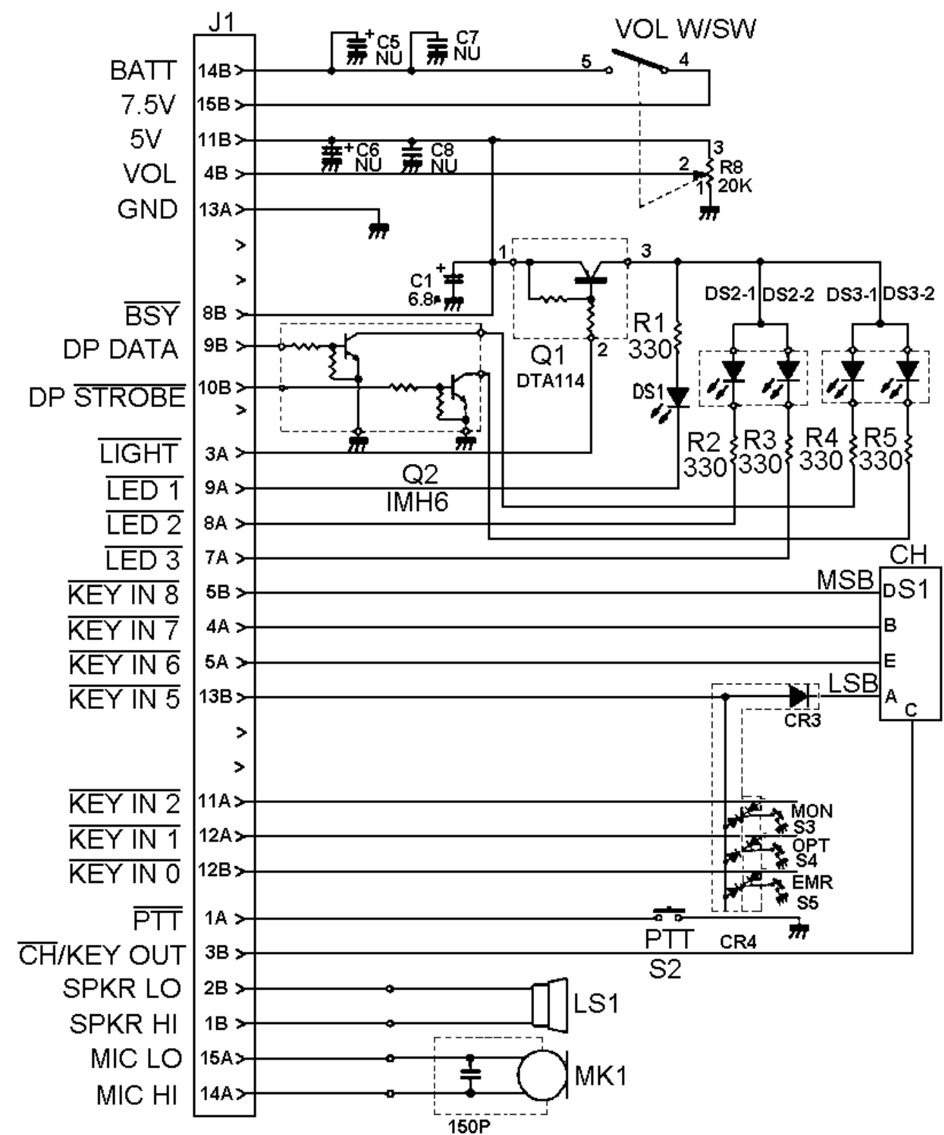
M-RK I (ANALOG) LED FLEX ASSEMBLY K19/AS00000040 (A3WE05285, Rev. 4)
