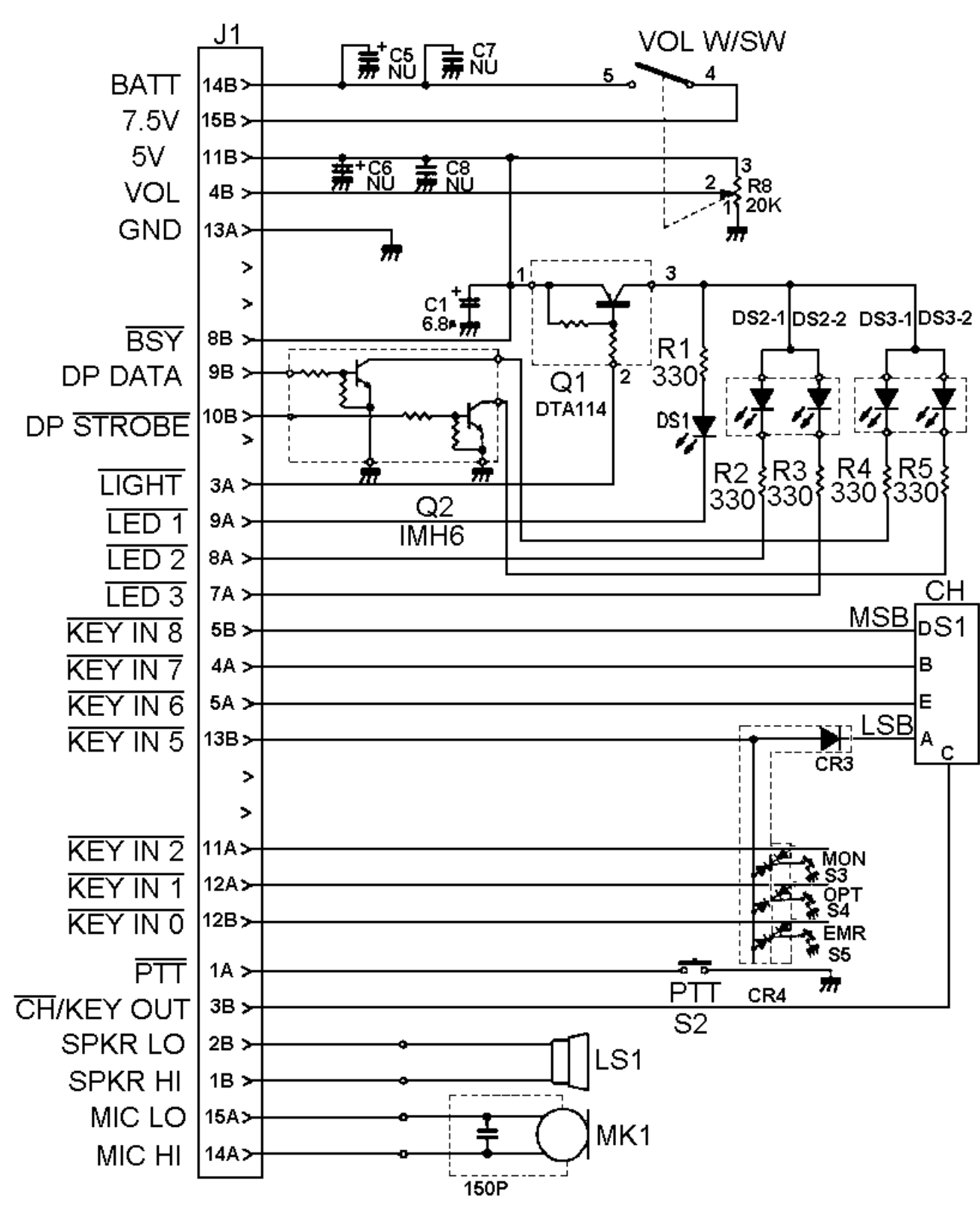
M-RK I (AEGIS) LED FLEX ASSEMBLY K19/AS00001121 (A4WE06081, Rev. 1)
