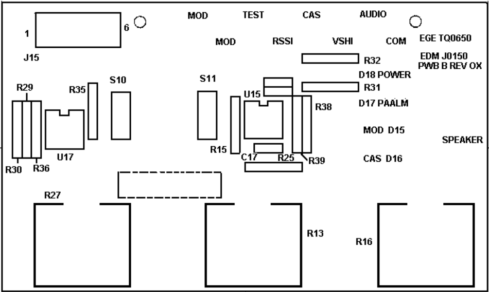
PRINTED WIRING BOARD B
