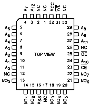
PLCC Package
