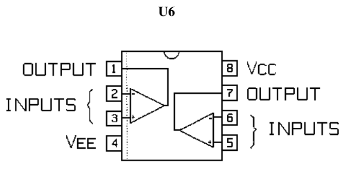
DUAL OP AMP 19A705798P1
