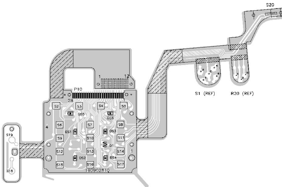
COMPONENT SIDE
