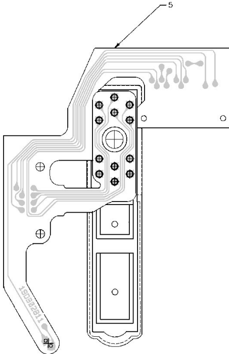
COMPONENT SIDE
